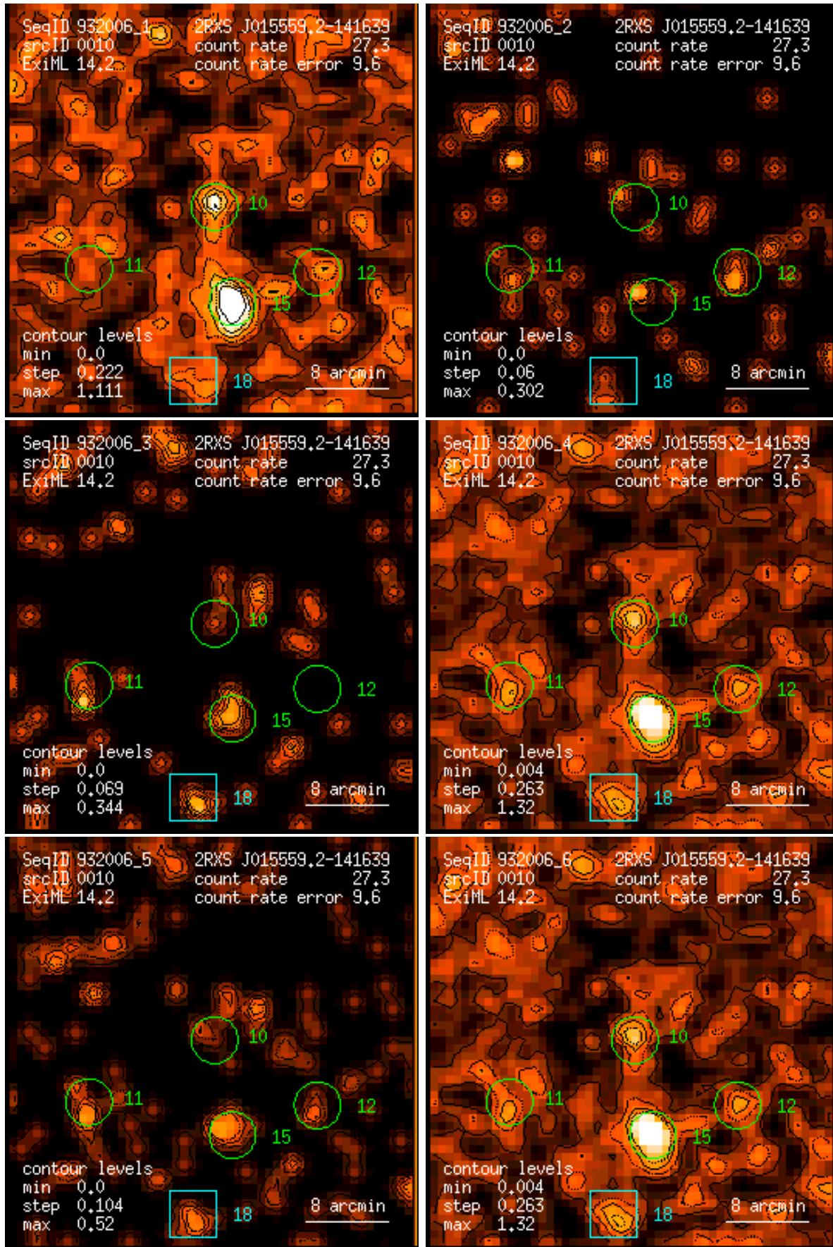
Figure 10: RASS 932006: detection 0010: band rate images, Gaussian filter: (1) PSPC channels 11 – 41, (2) 52 – 90, (3) 91 – 201, (4) 11 – 235, (5) 52 – 201, (6) 11 – 201. Broad band rates in counts/ks. Band rate contour levels in counts/ks/arcmin 2 .
