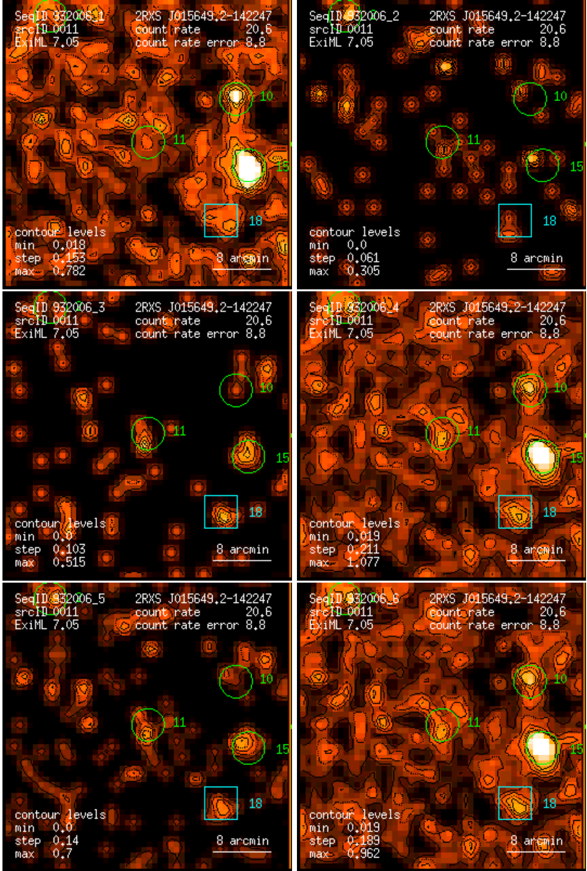
Figure 11: RASS 932006: detection 0011: band rate images, Gaussian filter: (1) PSPC channels 11 – 41, (2) 52 – 90, (3) 91 – 201, (4) 11 – 235, (5) 52 – 201, (6) 11 – 201. Broad band rates in counts/ks. Band rate contour levels in counts/ks/arcmin 2 .
