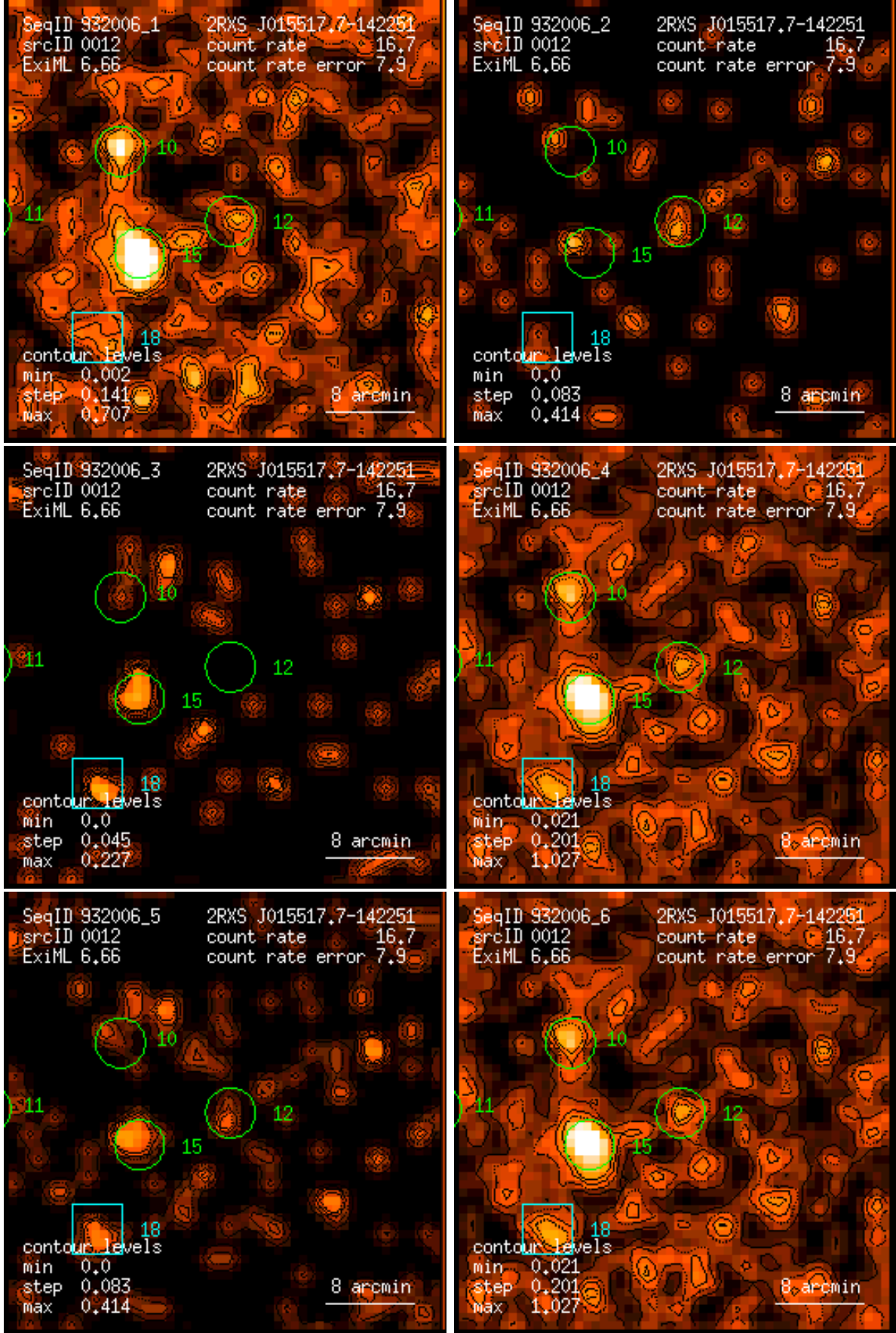
Figure 12: RASS 932006: detection 0012: band rate images, Gaussian filter: (1) PSPC channels 11 – 41, (2) 52 – 90, (3) 91 – 201, (4) 11 – 235, (5) 52 – 201, (6) 11 – 201. Broad band rates in counts/ks. Band rate contour levels in counts/ks/arcmin 2 .
