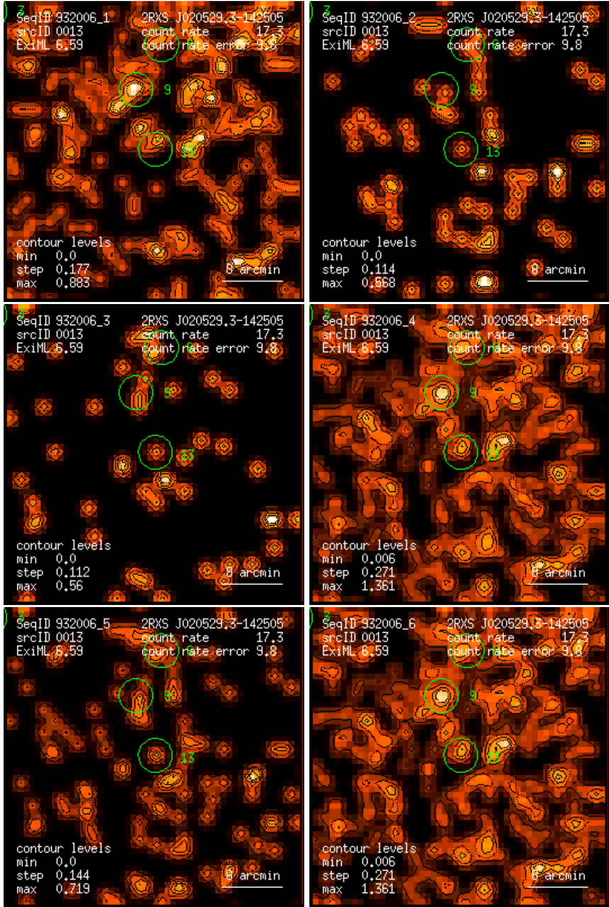
Figure 13: RASS 932006: detection 0013: band rate images, Gaussian filter: (1) PSPC channels 11 – 41, (2) 52 – 90, (3) 91 – 201, (4) 11 – 235, (5) 52 – 201, (6) 11 – 201. Broad band rates in counts/ks. Band rate contour levels in counts/ks/arcmin 2 .
