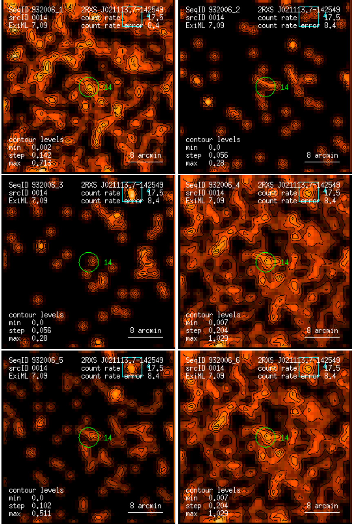
Figure 14: RASS 932006: detection 0014: band rate images, Gaussian filter: (1) PSPC channels 11 – 41, (2) 52 – 90, (3) 91 – 201, (4) 11 – 235, (5) 52 – 201, (6) 11 – 201. Broad band rates in counts/ks. Band rate contour levels in counts/ks/arcmin 2 .
