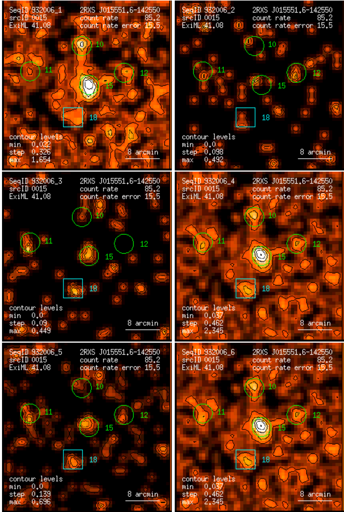
Figure 15: RASS 932006: detection 0015: band rate images, Gaussian filter: (1) PSPC channels 11 – 41, (2) 52 – 90, (3) 91 – 201, (4) 11 – 235, (5) 52 – 201, (6) 11 – 201. Broad band rates in counts/ks. Band rate contour levels in counts/ks/arcmin 2 .
