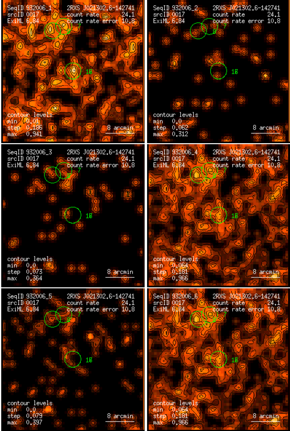
Figure 17: RASS 932006: detection 0017: band rate images, Gaussian filter: (1) PSPC channels 11 – 41, (2) 52 – 90, (3) 91 – 201, (4) 11 – 235, (5) 52 – 201, (6) 11 – 201. Broad band rates in counts/ks. Band rate contour levels in counts/ks/arcmin 2 .
