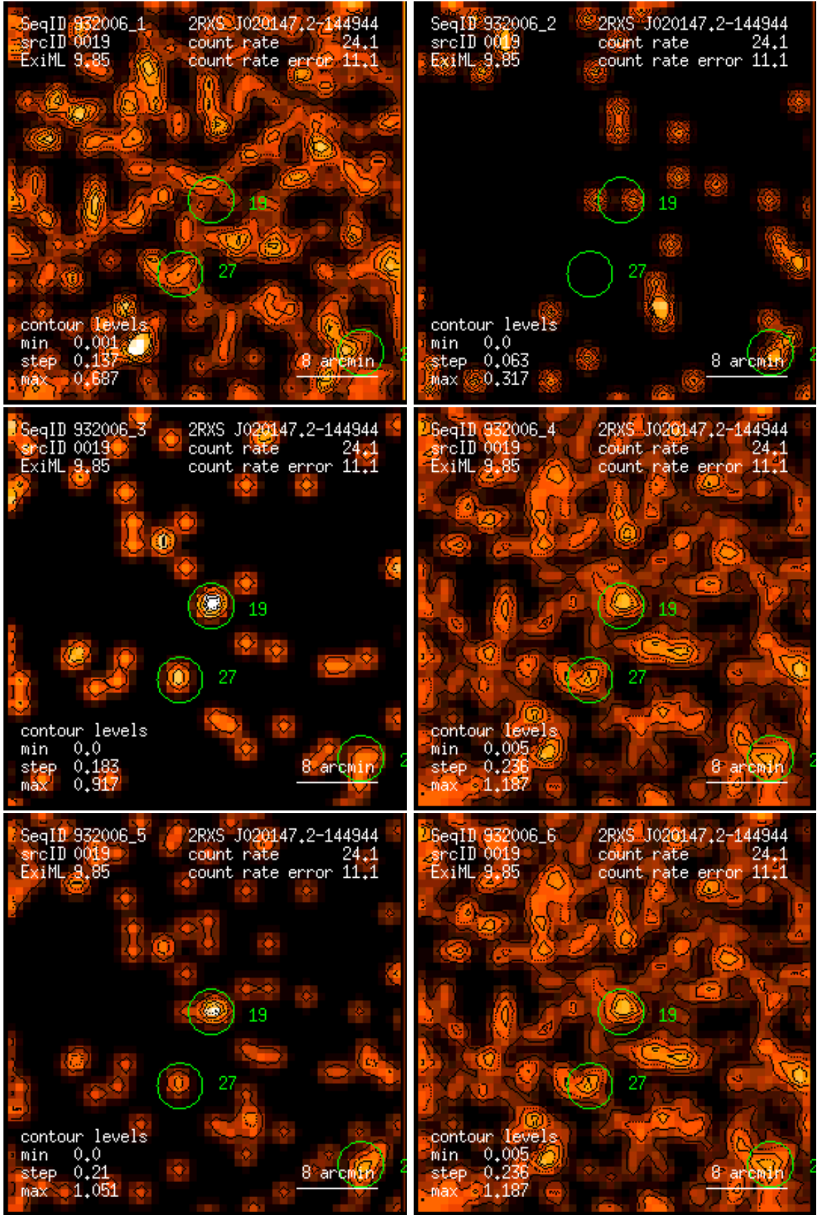
Figure 19: RASS 932006: detection 0019: band rate images, Gaussian filter: (1) PSPC channels 11 – 41, (2) 52 – 90, (3) 91 – 201, (4) 11 – 235, (5) 52 – 201, (6) 11 – 201. Broad band rates in counts/ks. Band rate contour levels in counts/ks/arcmin 2 .
