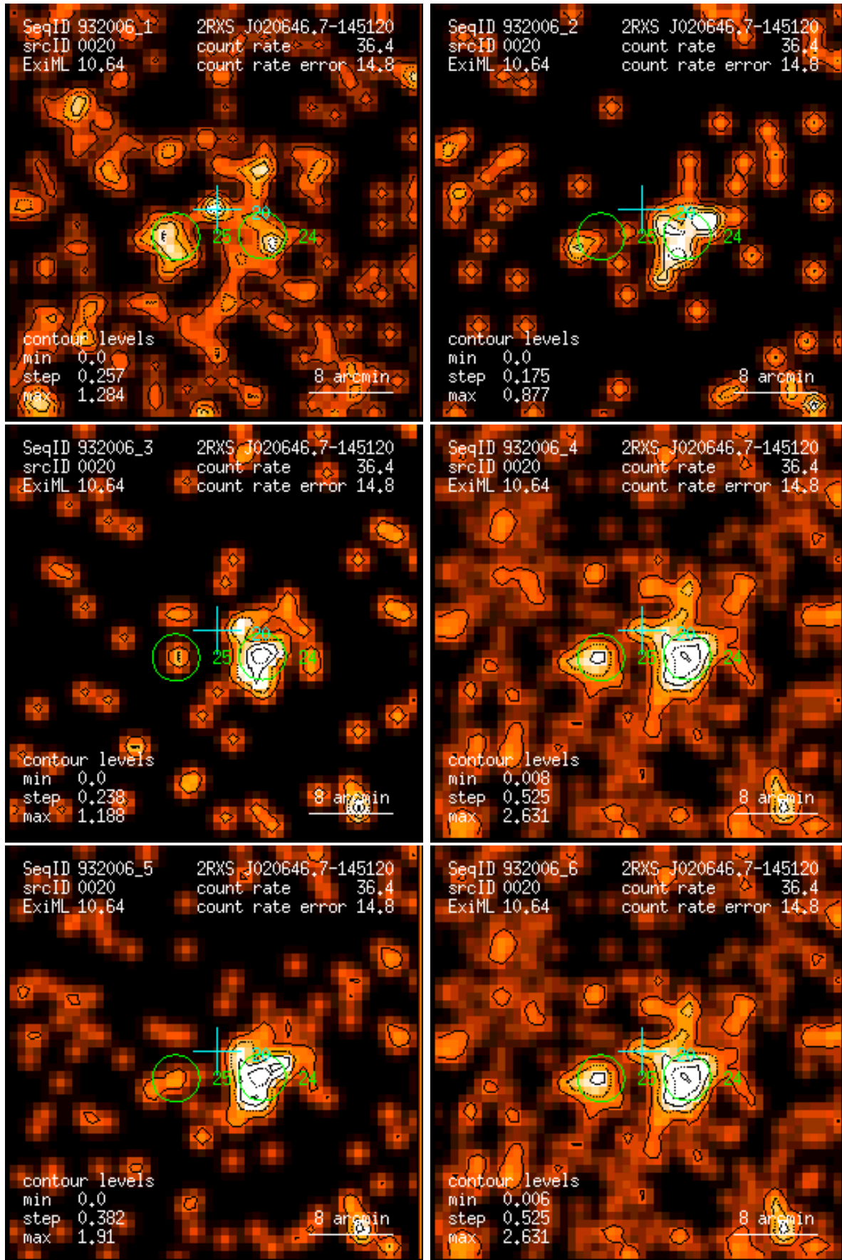
Figure 20: RASS 932006: detection 0020: band rate images, Gaussian filter: (1) PSPC channels 11 – 41, (2) 52 – 90, (3) 91 – 201, (4) 11 – 235, (5) 52 – 201, (6) 11 – 201. Broad band rates in counts/ks. Band rate contour levels in counts/ks/arcmin 2 .
