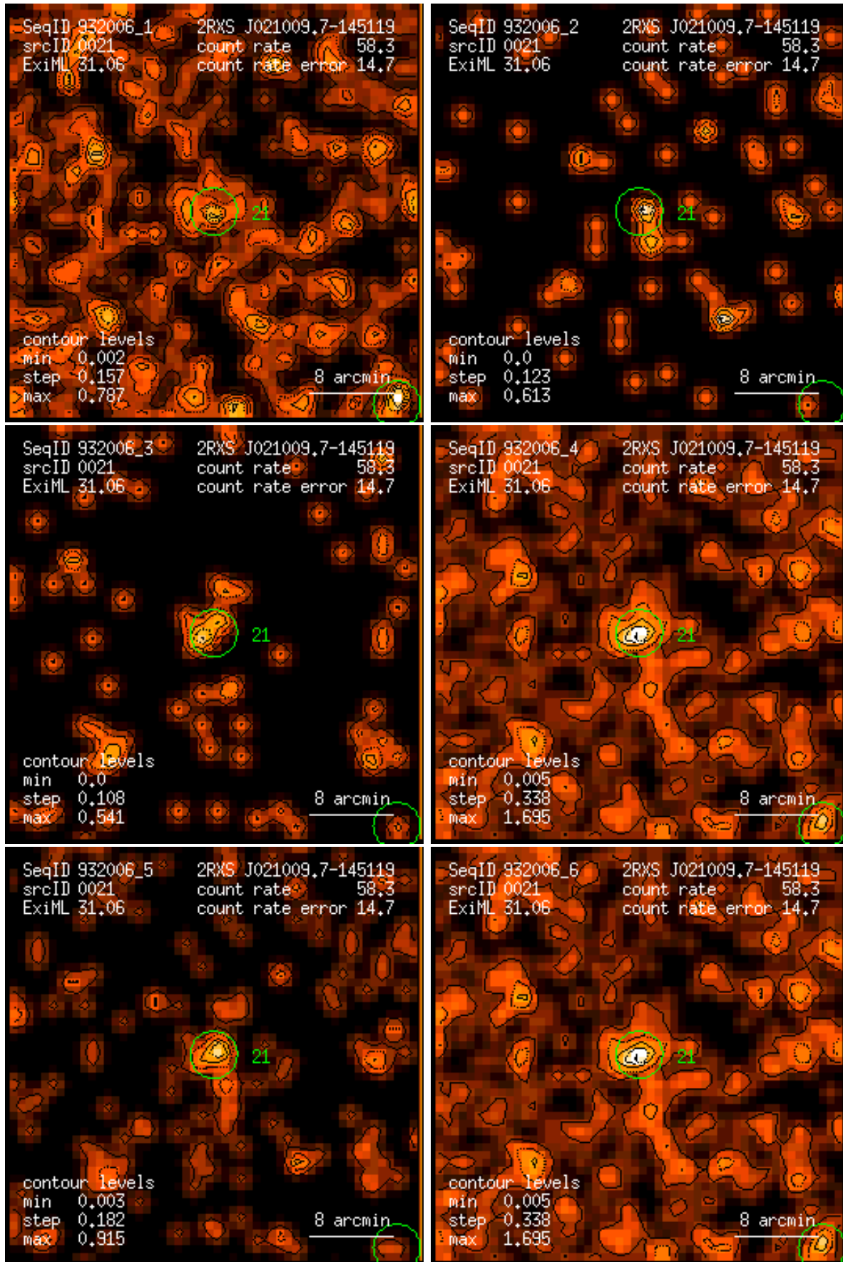
Figure 21: RASS 932006: detection 0021: band rate images, Gaussian filter: (1) PSPC channels 11 – 41, (2) 52 – 90, (3) 91 – 201, (4) 11 – 235, (5) 52 – 201, (6) 11 – 201. Broad band rates in counts/ks. Band rate contour levels in counts/ks/arcmin 2 .
