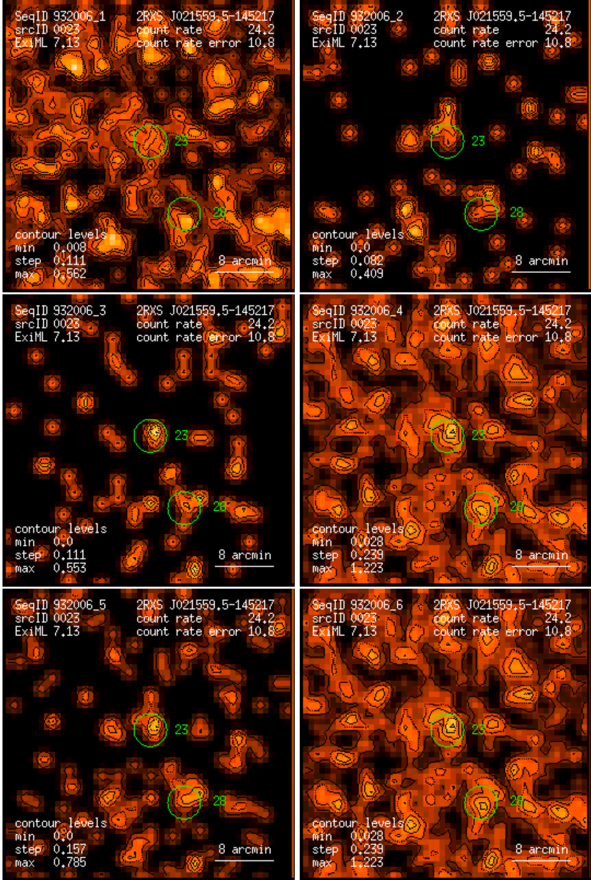
Figure 23: RASS 932006: detection 0023: band rate images, Gaussian filter: (1) PSPC channels 11 – 41, (2) 52 – 90, (3) 91 – 201, (4) 11 – 235, (5) 52 – 201, (6) 11 – 201. Broad band rates in counts/ks. Band rate contour levels in counts/ks/arcmin 2 .
