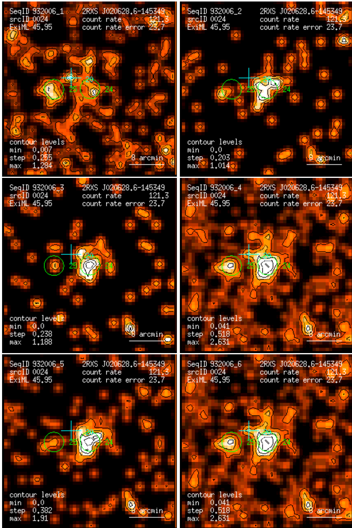
Figure 24: RASS 932006: detection 0024: band rate images, Gaussian filter: (1) PSPC channels 11 – 41, (2) 52 – 90, (3) 91 – 201, (4) 11 – 235, (5) 52 – 201, (6) 11 – 201. Broad band rates in counts/ks. Band rate contour levels in counts/ks/arcmin 2 .
