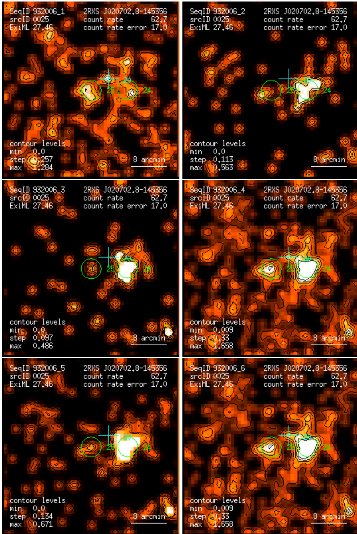
Figure 25: RASS 932006: detection 0025: band rate images, Gaussian filter: (1) PSPC channels 11 – 41, (2) 52 – 90, (3) 91 – 201, (4) 11 – 235, (5) 52 – 201, (6) 11 – 201. Broad band rates in counts/ks. Band rate contour levels in counts/ks/arcmin 2 .
