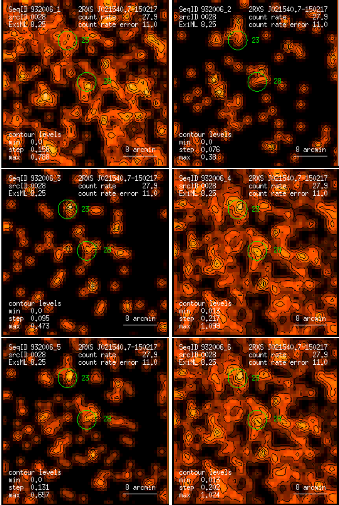
Figure 28: RASS 932006: detection 0028: band rate images, Gaussian filter: (1) PSPC channels 11 – 41, (2) 52 – 90, (3) 91 – 201, (4) 11 – 235, (5) 52 – 201, (6) 11 – 201. Broad band rates in counts/ks. Band rate contour levels in counts/ks/arcmin 2 .
