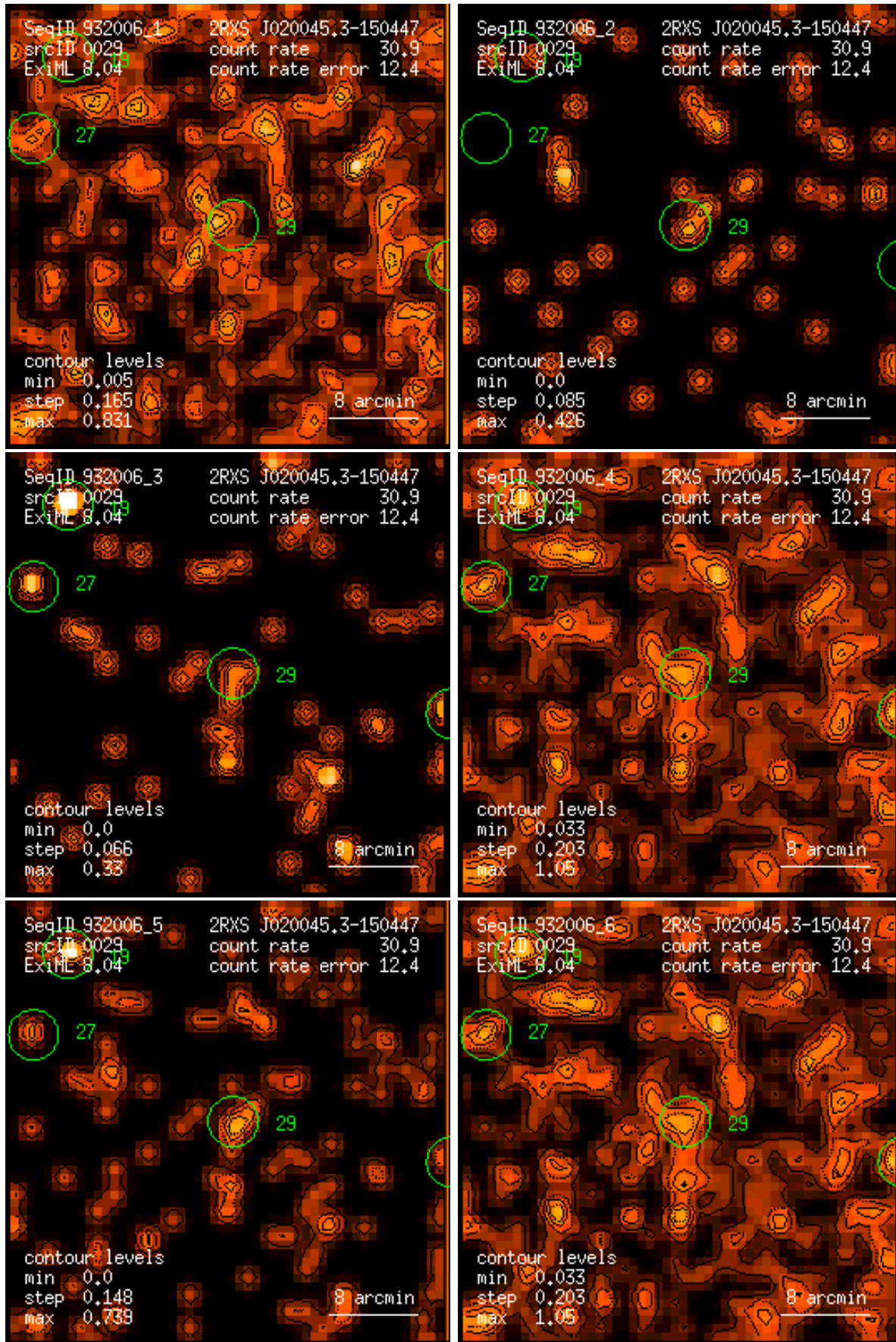
Figure 29: RASS 932006: detection 0029: band rate images, Gaussian filter: (1) PSPC channels 11 – 41, (2) 52 – 90, (3) 91 – 201, (4) 11 – 235, (5) 52 – 201, (6) 11 – 201. Broad band rates in counts/ks. Band rate contour levels in counts/ks/arcmin 2 .
