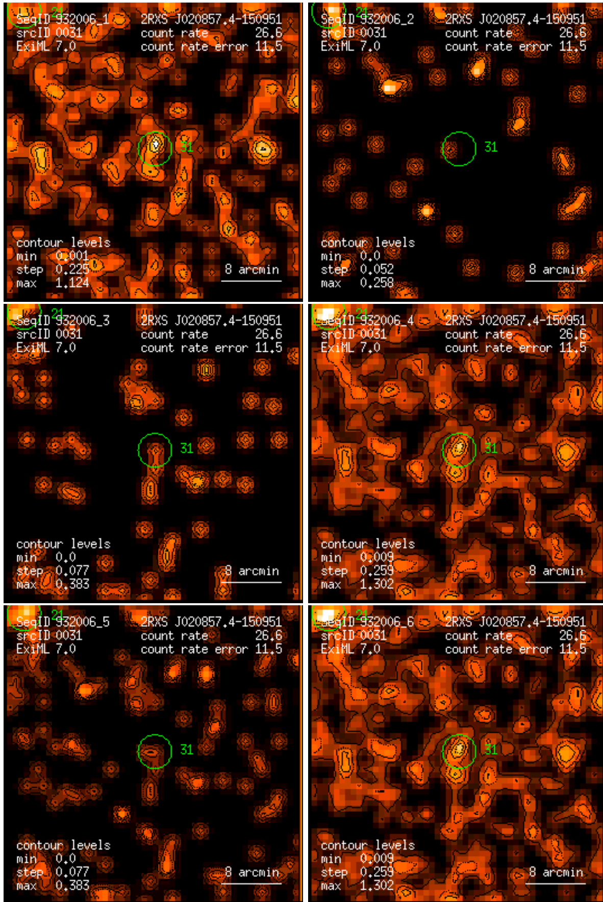
Figure 31: RASS 932006: detection 0031: band rate images, Gaussian filter: (1) PSPC channels 11 – 41, (2) 52 – 90, (3) 91 – 201, (4) 11 – 235, (5) 52 – 201, (6) 11 – 201. Broad band rates in counts/ks. Band rate contour levels in counts/ks/arcmin 2 .
