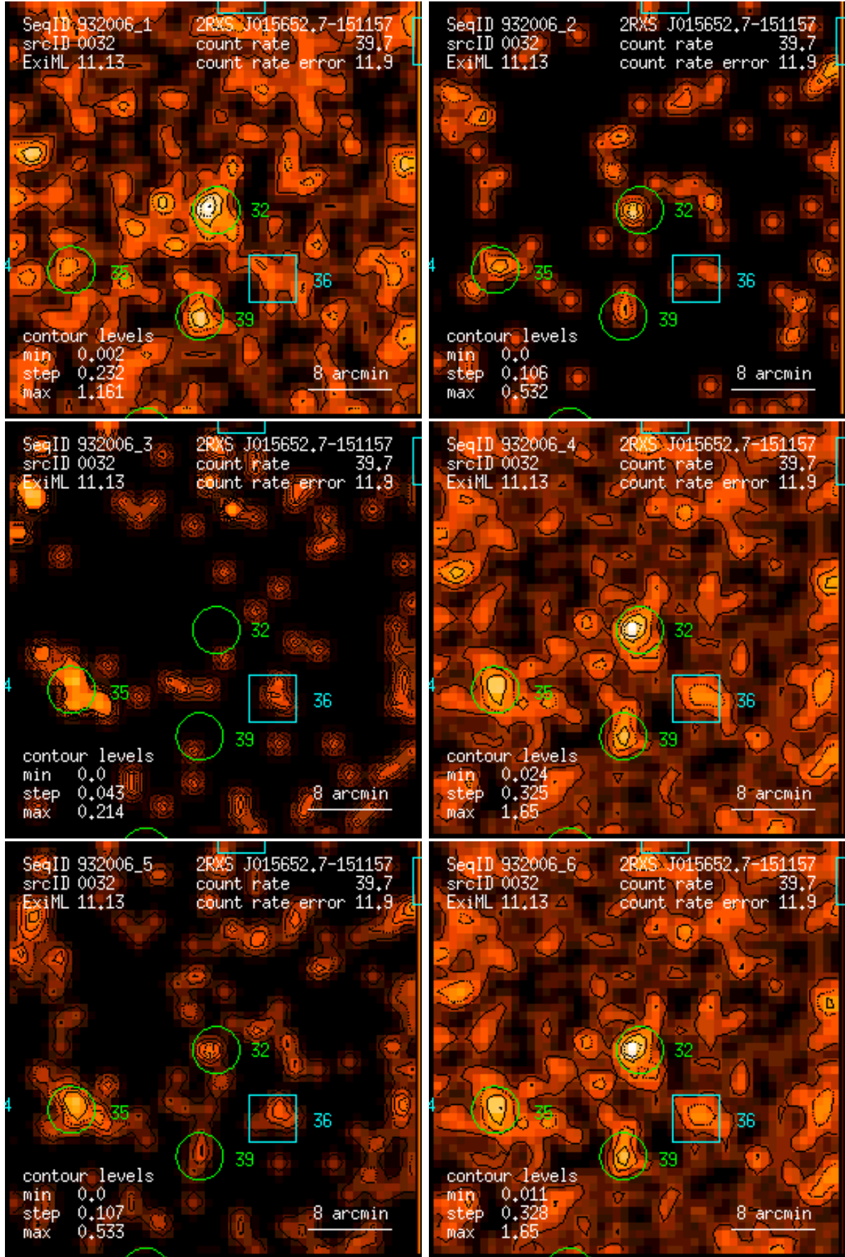
Figure 32: RASS 932006: detection 0032: band rate images, Gaussian filter: (1) PSPC channels 11 – 41, (2) 52 – 90, (3) 91 – 201, (4) 11 – 235, (5) 52 – 201, (6) 11 – 201. Broad band rates in counts/ks. Band rate contour levels in counts/ks/arcmin 2 .
