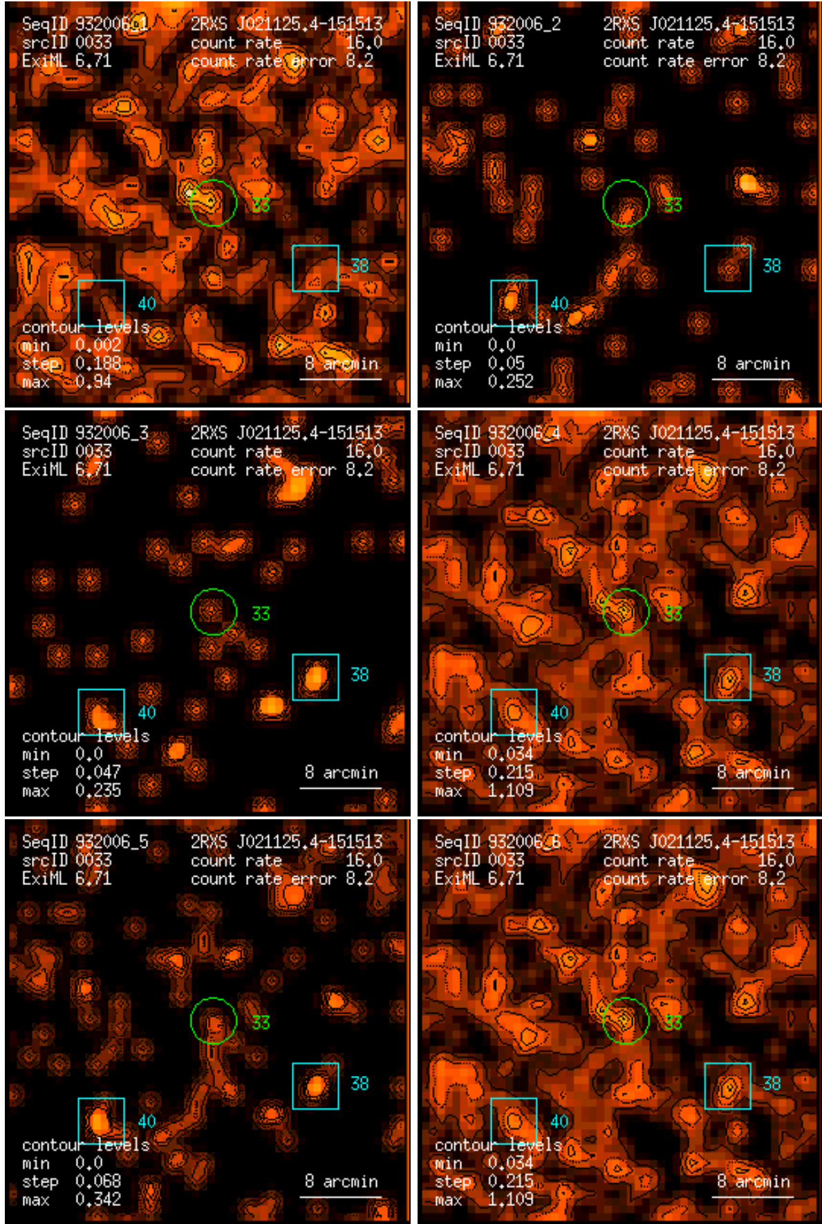
Figure 33: RASS 932006: detection 0033: band rate images, Gaussian filter: (1) PSPC channels 11 – 41, (2) 52 – 90, (3) 91 – 201, (4) 11 – 235, (5) 52 – 201, (6) 11 – 201. Broad band rates in counts/ks. Band rate contour levels in counts/ks/arcmin 2 .
