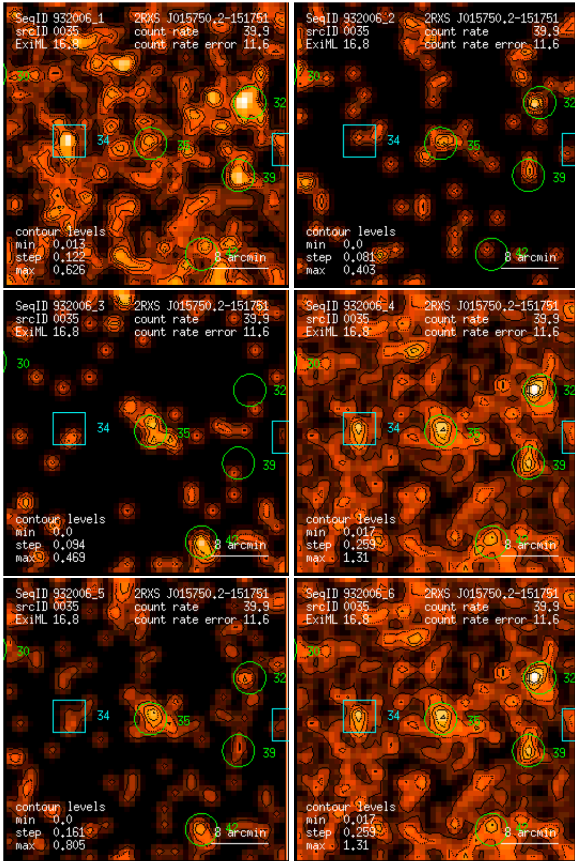
Figure 35: RASS 932006: detection 0035: band rate images, Gaussian filter: (1) PSPC channels 11 – 41, (2) 52 – 90, (3) 91 – 201, (4) 11 – 235, (5) 52 – 201, (6) 11 – 201. Broad band rates in counts/ks. Band rate contour levels in counts/ks/arcmin 2 .
