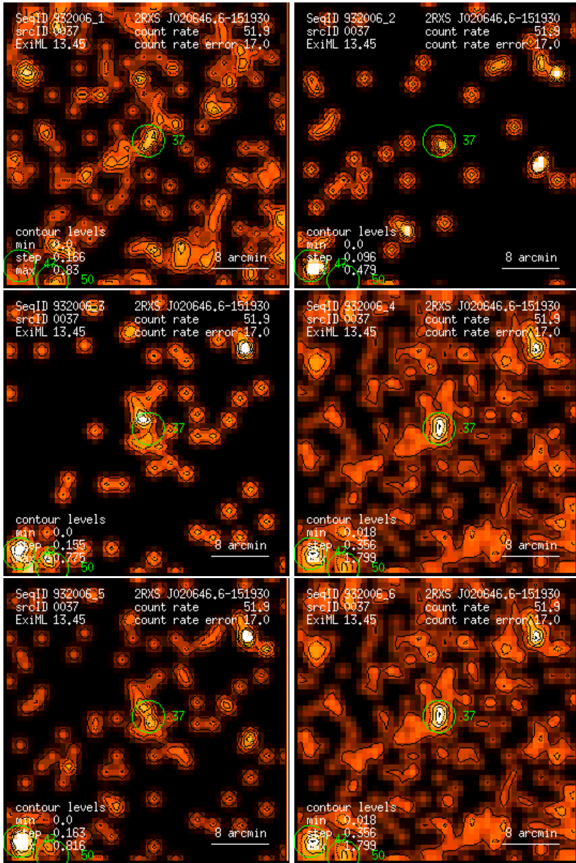
Figure 37: RASS 932006: detection 0037: band rate images, Gaussian filter: (1) PSPC channels 11 – 41, (2) 52 – 90, (3) 91 – 201, (4) 11 – 235, (5) 52 – 201, (6) 11 – 201. Broad band rates in counts/ks. Band rate contour levels in counts/ks/arcmin 2 .
