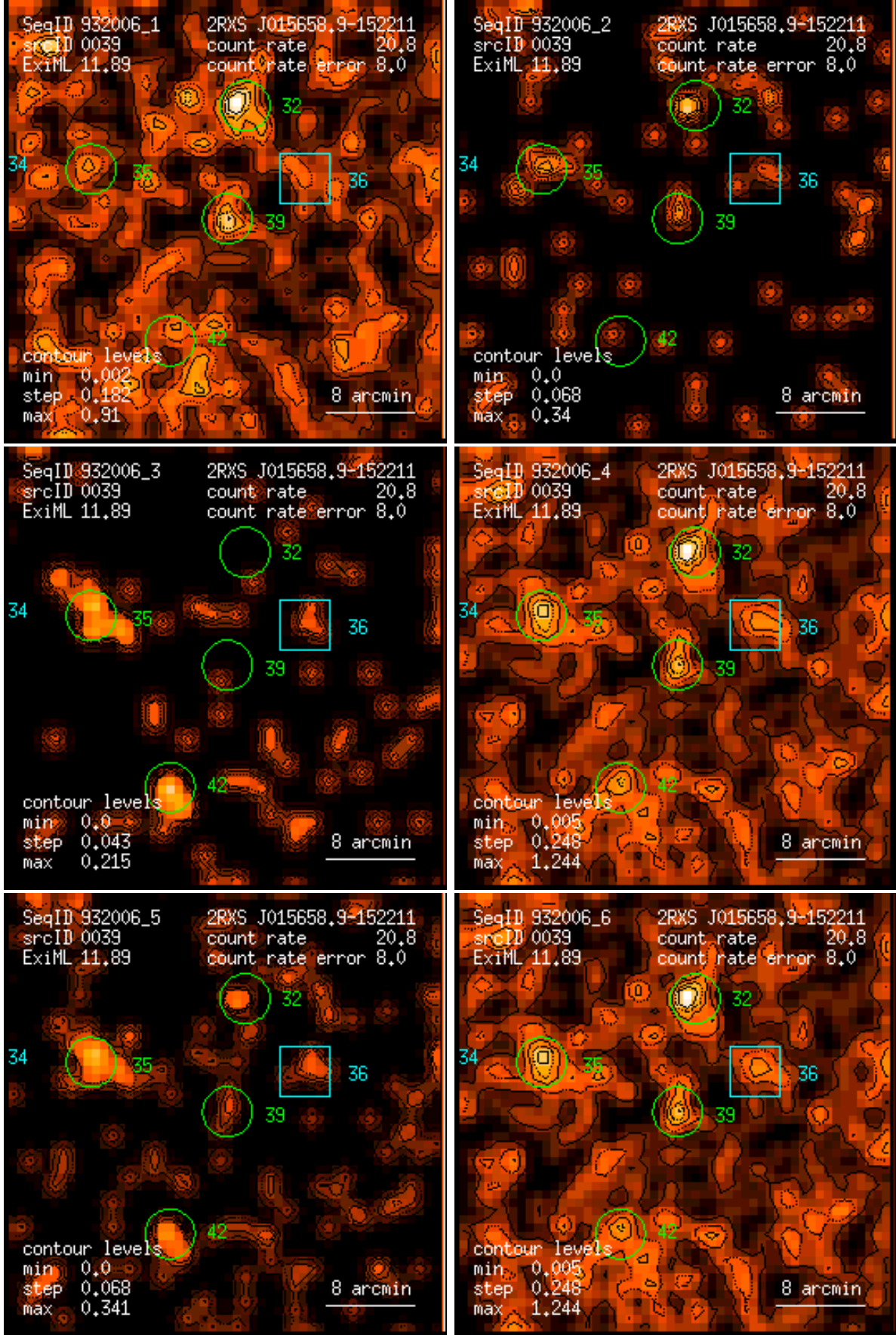
Figure 39: RASS 932006: detection 0039: band rate images, Gaussian filter: (1) PSPC channels 11 – 41, (2) 52 – 90, (3) 91 – 201, (4) 11 – 235, (5) 52 – 201, (6) 11 – 201. Broad band rates in counts/ks. Band rate contour levels in counts/ks/arcmin 2 .
