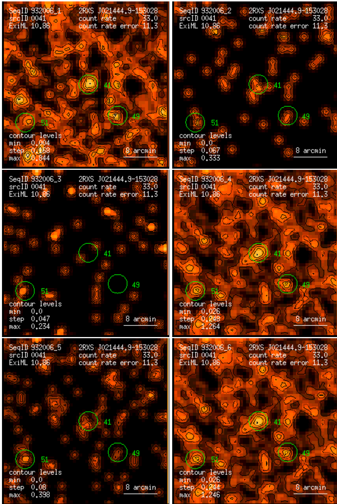
Figure 41: RASS 932006: detection 0041: band rate images, Gaussian filter: (1) PSPC channels 11 – 41, (2) 52 – 90, (3) 91 – 201, (4) 11 – 235, (5) 52 – 201, (6) 11 – 201. Broad band rates in counts/ks. Band rate contour levels in counts/ks/arcmin 2 .
