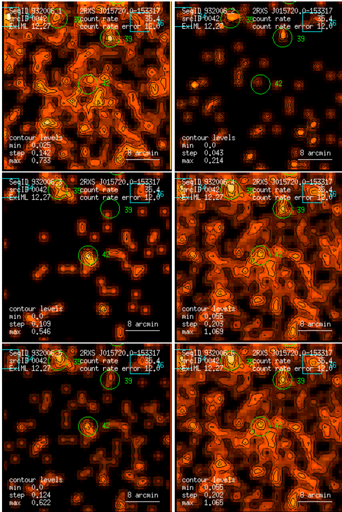
Figure 42: RASS 932006: detection 0042: band rate images, Gaussian filter: (1) PSPC channels 11 – 41, (2) 52 – 90, (3) 91 – 201, (4) 11 – 235, (5) 52 – 201, (6) 11 – 201. Broad band rates in counts/ks. Band rate contour levels in counts/ks/arcmin 2 .
