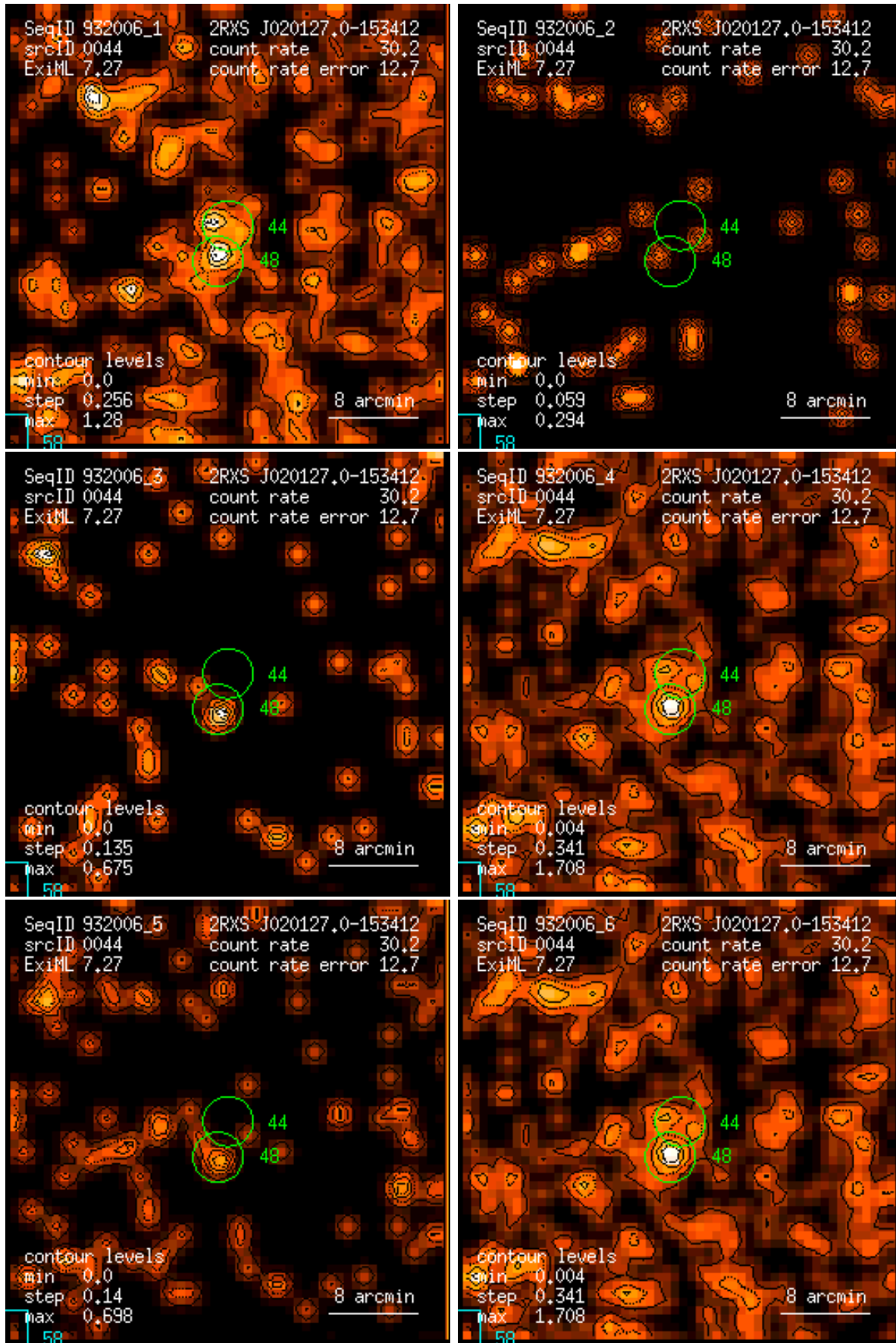
Figure 44: RASS 932006: detection 0044: band rate images, Gaussian filter: (1) PSPC channels 11 – 41, (2) 52 – 90, (3) 91 – 201, (4) 11 – 235, (5) 52 – 201, (6) 11 – 201. Broad band rates in counts/ks. Band rate contour levels in counts/ks/arcmin 2 .
