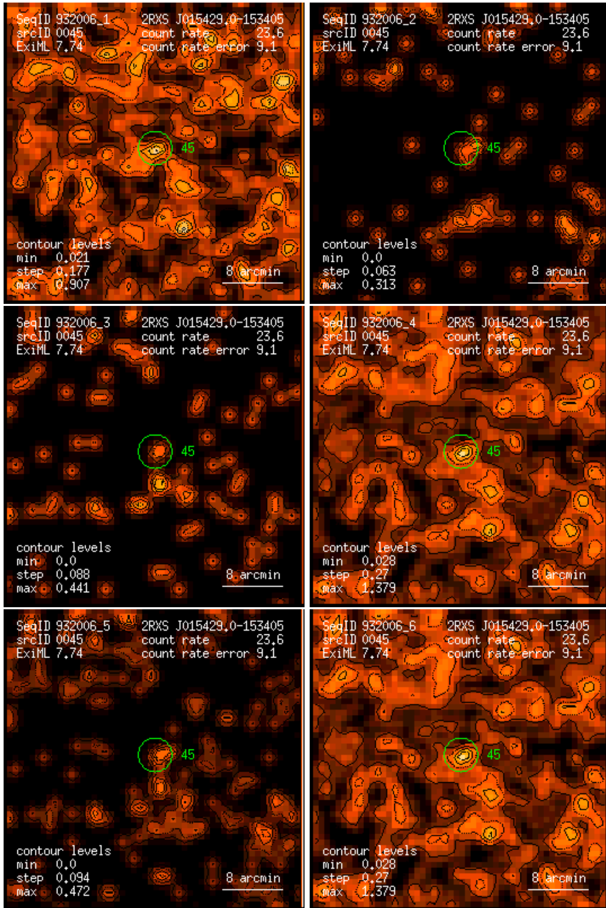
Figure 45: RASS 932006: detection 0045: band rate images, Gaussian filter: (1) PSPC channels 11 – 41, (2) 52 – 90, (3) 91 – 201, (4) 11 – 235, (5) 52 – 201, (6) 11 – 201. Broad band rates in counts/ks. Band rate contour levels in counts/ks/arcmin 2 .
