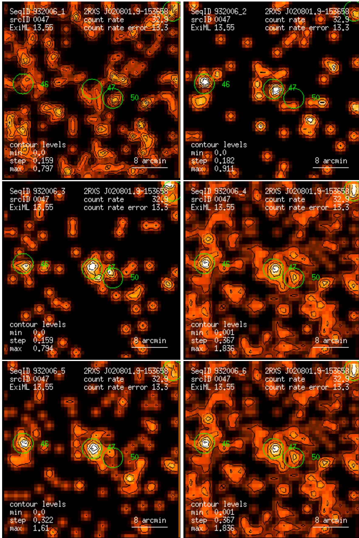
Figure 47: RASS 932006: detection 0047: band rate images, Gaussian filter: (1) PSPC channels 11 – 41, (2) 52 – 90, (3) 91 – 201, (4) 11 – 235, (5) 52 – 201, (6) 11 – 201. Broad band rates in counts/ks. Band rate contour levels in counts/ks/arcmin 2 .
