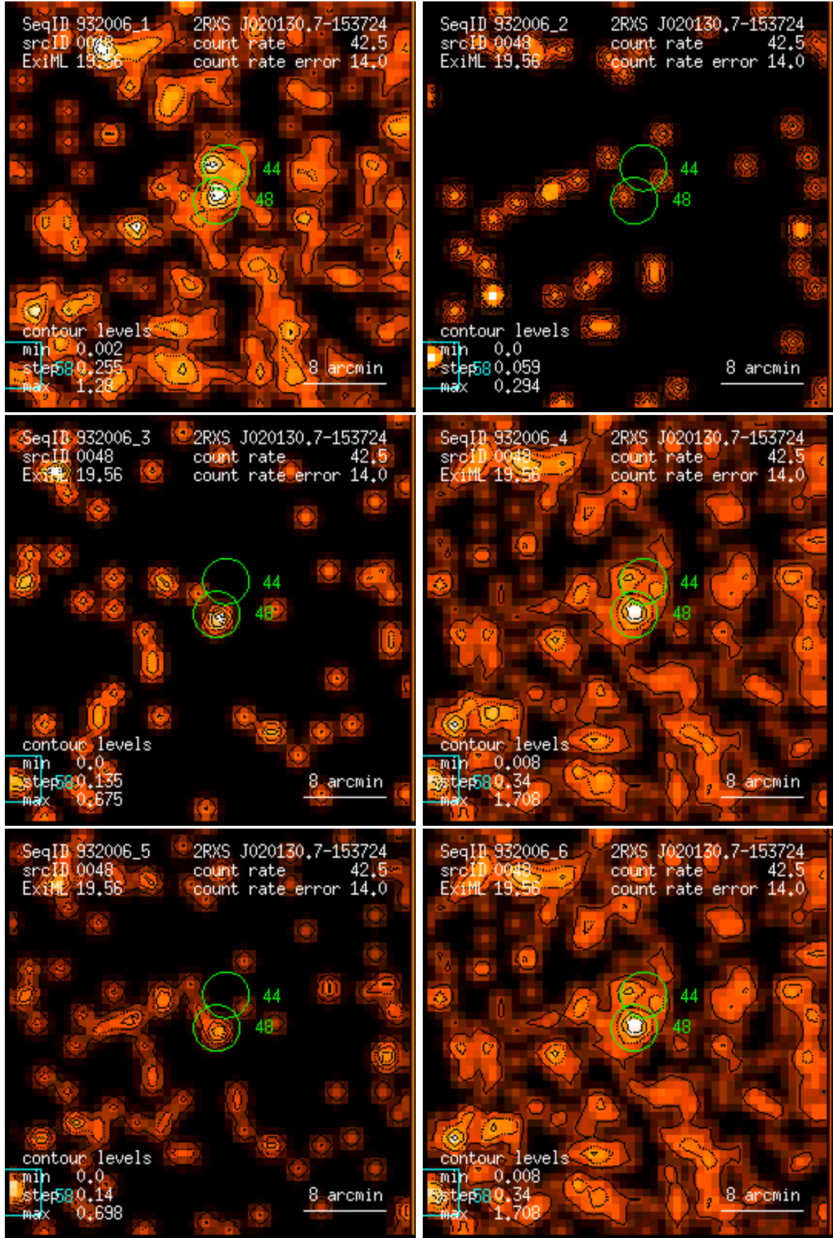
Figure 48: RASS 932006: detection 0048: band rate images, Gaussian filter: (1) PSPC channels 11 – 41, (2) 52 – 90, (3) 91 – 201, (4) 11 – 235, (5) 52 – 201, (6) 11 – 201. Broad band rates in counts/ks. Band rate contour levels in counts/ks/arcmin 2 .
