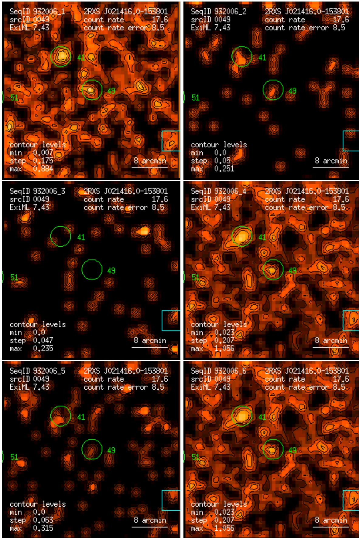
Figure 49: RASS 932006: detection 0049: band rate images, Gaussian filter: (1) PSPC channels 11 – 41, (2) 52 – 90, (3) 91 – 201, (4) 11 – 235, (5) 52 – 201, (6) 11 – 201. Broad band rates in counts/ks. Band rate contour levels in counts/ks/arcmin 2 .
