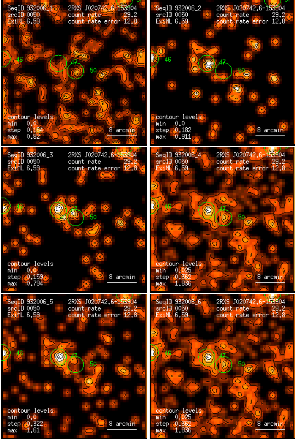
Figure 50: RASS 932006: detection 0050: band rate images, Gaussian filter: (1) PSPC channels 11 – 41, (2) 52 – 90, (3) 91 – 201, (4) 11 – 235, (5) 52 – 201, (6) 11 – 201. Broad band rates in counts/ks. Band rate contour levels in counts/ks/arcmin 2 .
