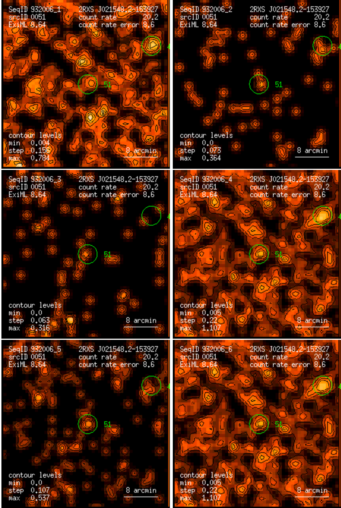
Figure 51: RASS 932006: detection 0051: band rate images, Gaussian filter: (1) PSPC channels 11 – 41, (2) 52 – 90, (3) 91 – 201, (4) 11 – 235, (5) 52 – 201, (6) 11 – 201. Broad band rates in counts/ks. Band rate contour levels in counts/ks/arcmin 2 .
