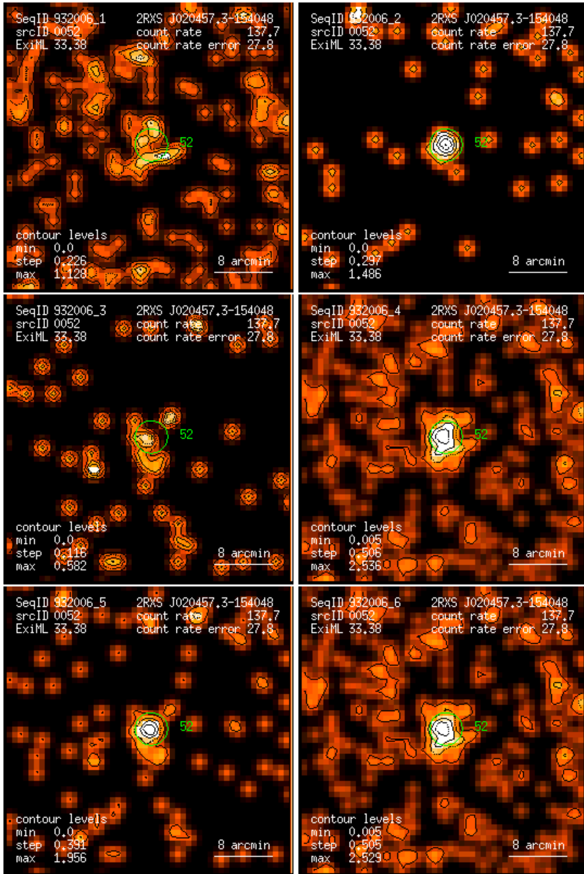
Figure 52: RASS 932006: detection 0052: band rate images, Gaussian filter: (1) PSPC channels 11 – 41, (2) 52 – 90, (3) 91 – 201, (4) 11 – 235, (5) 52 – 201, (6) 11 – 201. Broad band rates in counts/ks. Band rate contour levels in counts/ks/arcmin 2 .
