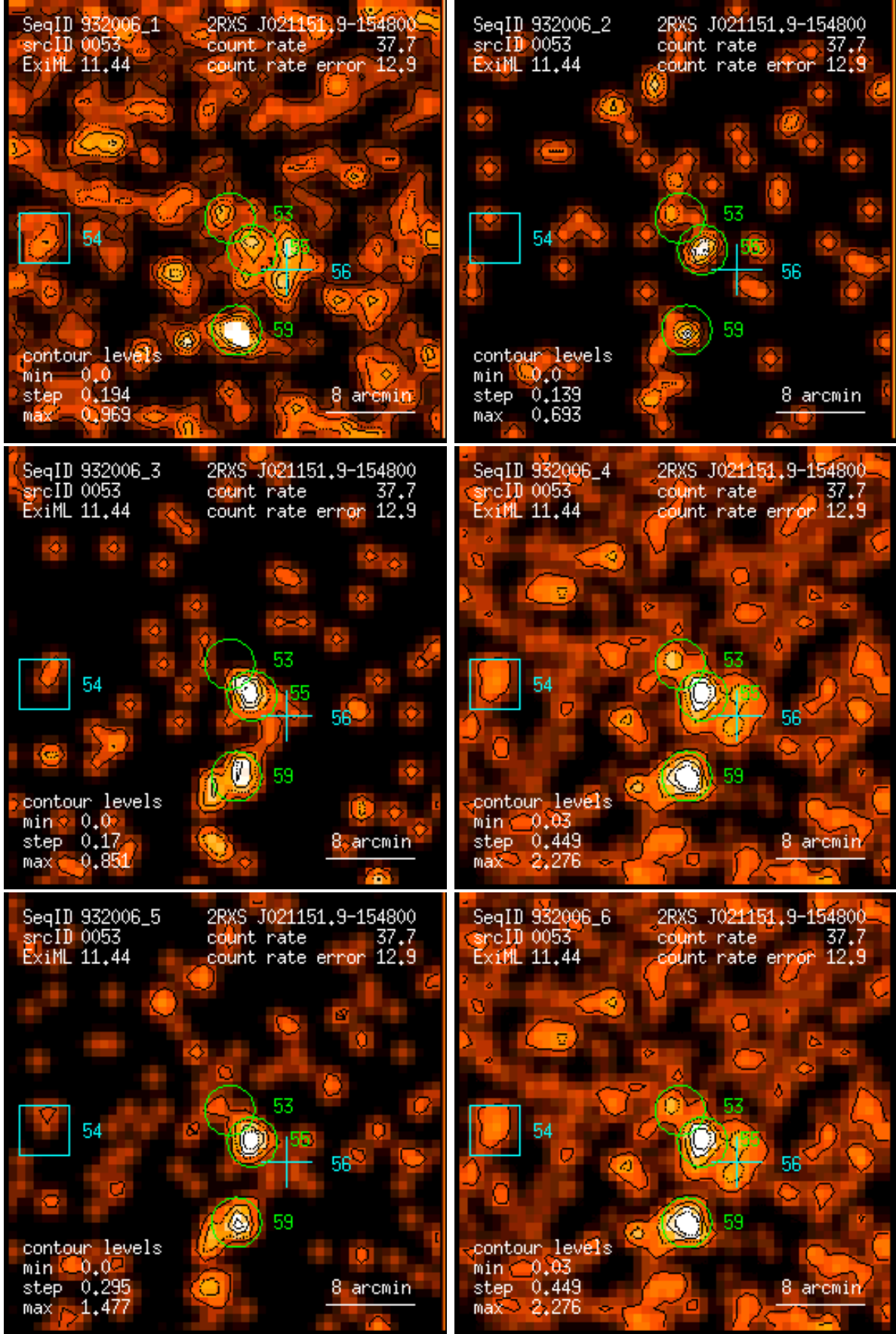
Figure 53: RASS 932006: detection 0053: band rate images, Gaussian filter: (1) PSPC channels 11 – 41, (2) 52 – 90, (3) 91 – 201, (4) 11 – 235, (5) 52 – 201, (6) 11 – 201. Broad band rates in counts/ks. Band rate contour levels in counts/ks/arcmin 2 .
