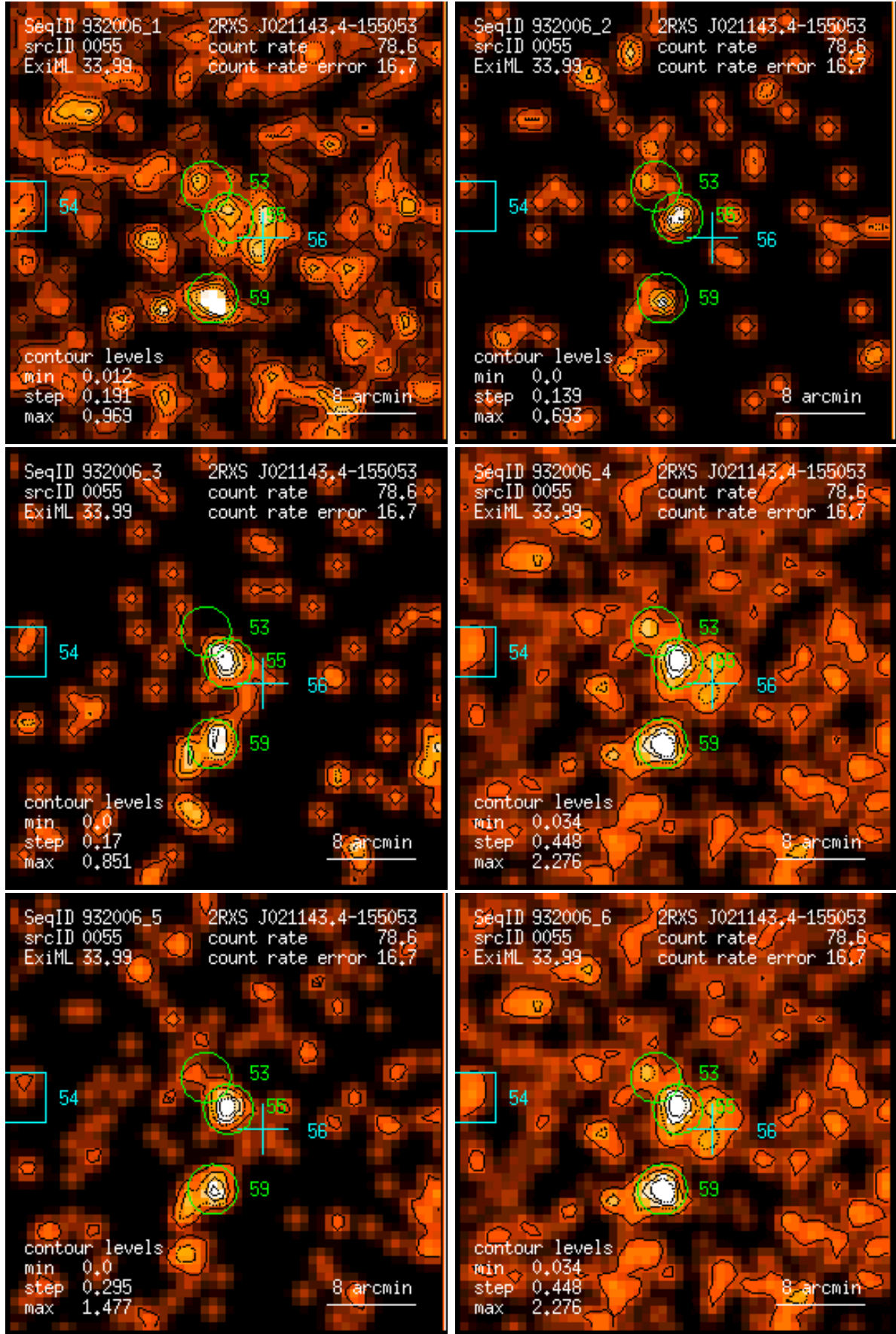
Figure 55: RASS 932006: detection 0055: band rate images, Gaussian filter: (1) PSPC channels 11 – 41, (2) 52 – 90, (3) 91 – 201, (4) 11 – 235, (5) 52 – 201, (6) 11 – 201. Broad band rates in counts/ks. Band rate contour levels in counts/ks/arcmin 2 .
