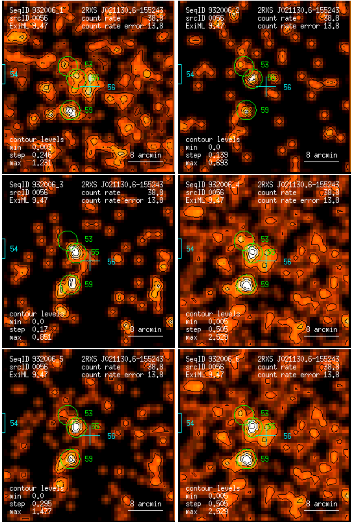
Figure 56: RASS 932006: detection 0056: band rate images, Gaussian filter: (1) PSPC channels 11 – 41, (2) 52 – 90, (3) 91 – 201, (4) 11 – 235, (5) 52 – 201, (6) 11 – 201. Broad band rates in counts/ks. Band rate contour levels in counts/ks/arcmin 2 .
