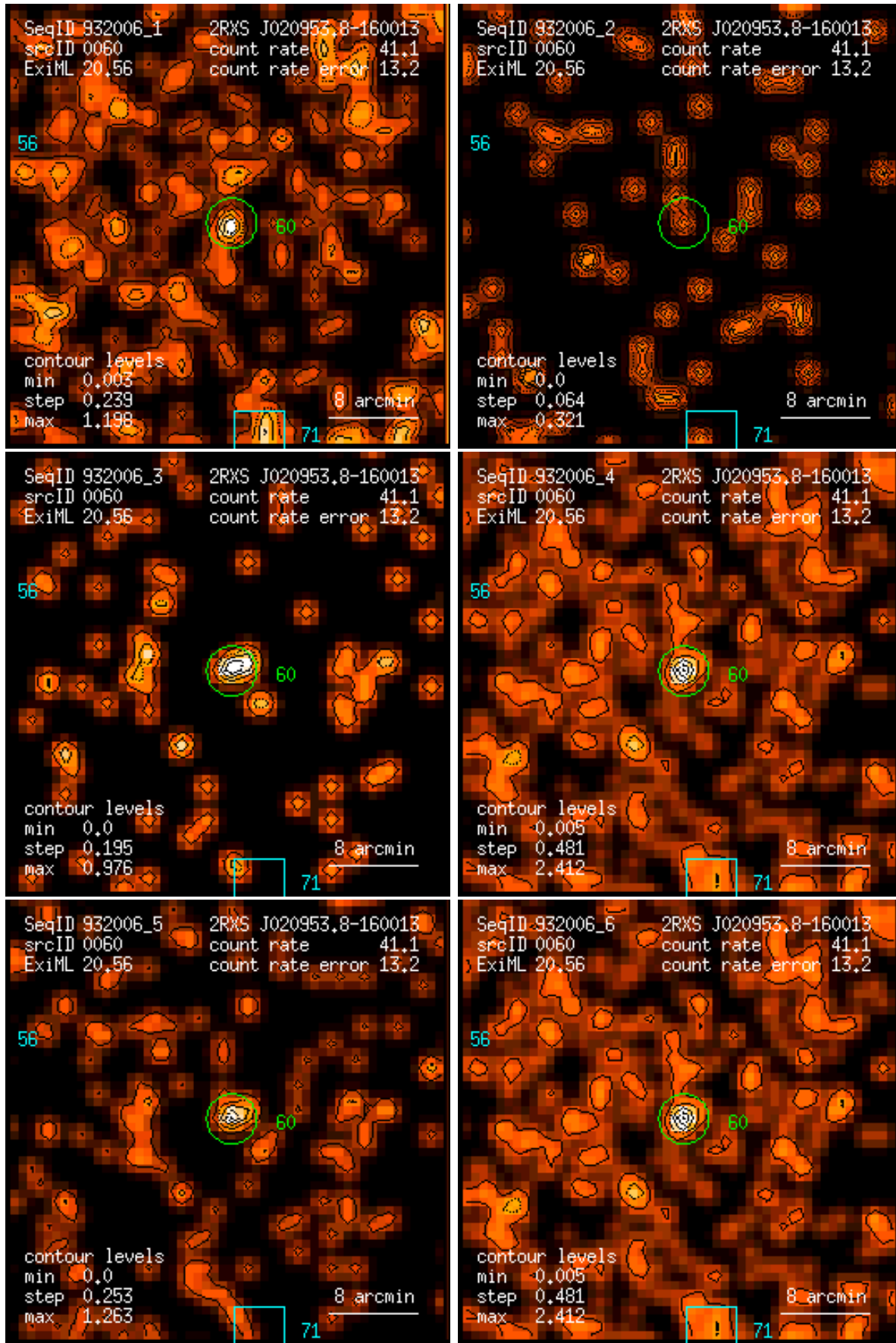
Figure 60: RASS 932006: detection 0060: band rate images, Gaussian filter: (1) PSPC channels 11 – 41, (2) 52 – 90, (3) 91 – 201, (4) 11 – 235, (5) 52 – 201, (6) 11 – 201. Broad band rates in counts/ks. Band rate contour levels in counts/ks/arcmin 2 .
