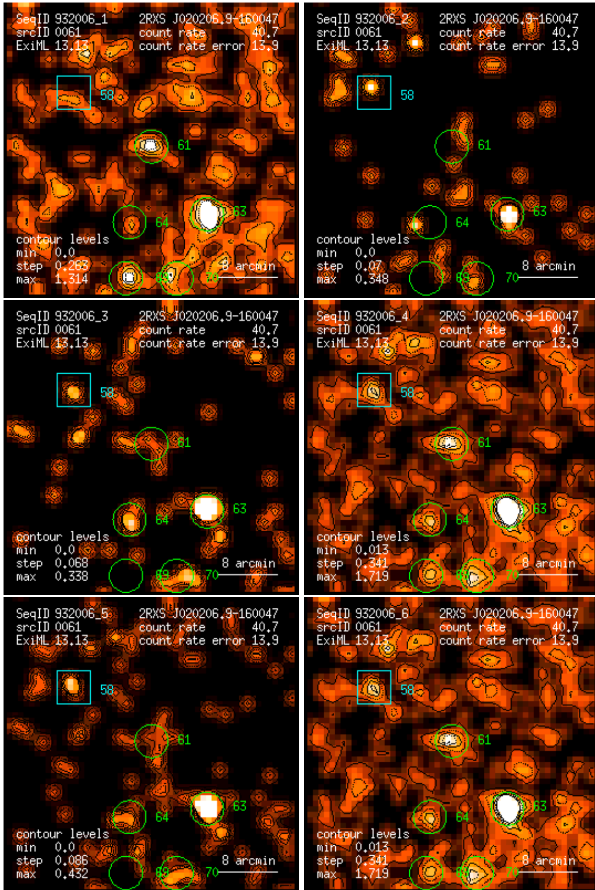
Figure 61: RASS 932006: detection 0061: band rate images, Gaussian filter: (1) PSPC channels 11 – 41, (2) 52 – 90, (3) 91 – 201, (4) 11 – 235, (5) 52 – 201, (6) 11 – 201. Broad band rates in counts/ks. Band rate contour levels in counts/ks/arcmin 2 .
