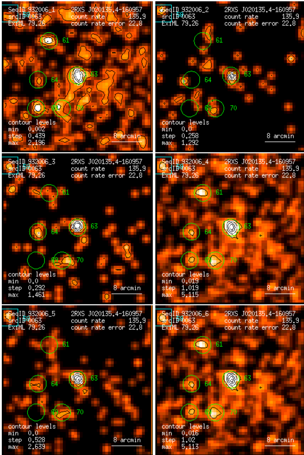
Figure 63: RASS 932006: detection 0063: band rate images, Gaussian filter: (1) PSPC channels 11 – 41, (2) 52 – 90, (3) 91 – 201, (4) 11 – 235, (5) 52 – 201, (6) 11 – 201. Broad band rates in counts/ks. Band rate contour levels in counts/ks/arcmin 2 .
