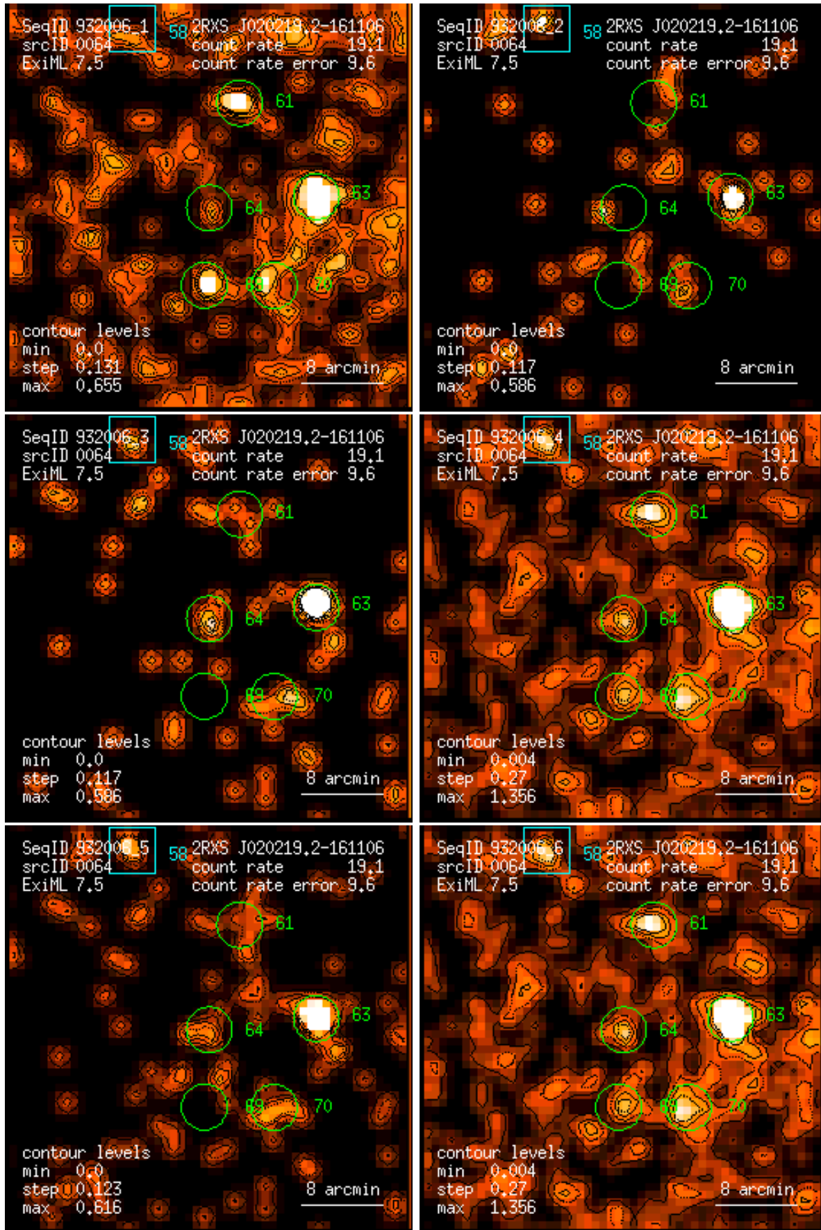
Figure 64: RASS 932006: detection 0064: band rate images, Gaussian filter: (1) PSPC channels 11 – 41, (2) 52 – 90, (3) 91 – 201, (4) 11 – 235, (5) 52 – 201, (6) 11 – 201. Broad band rates in counts/ks. Band rate contour levels in counts/ks/arcmin 2 .
