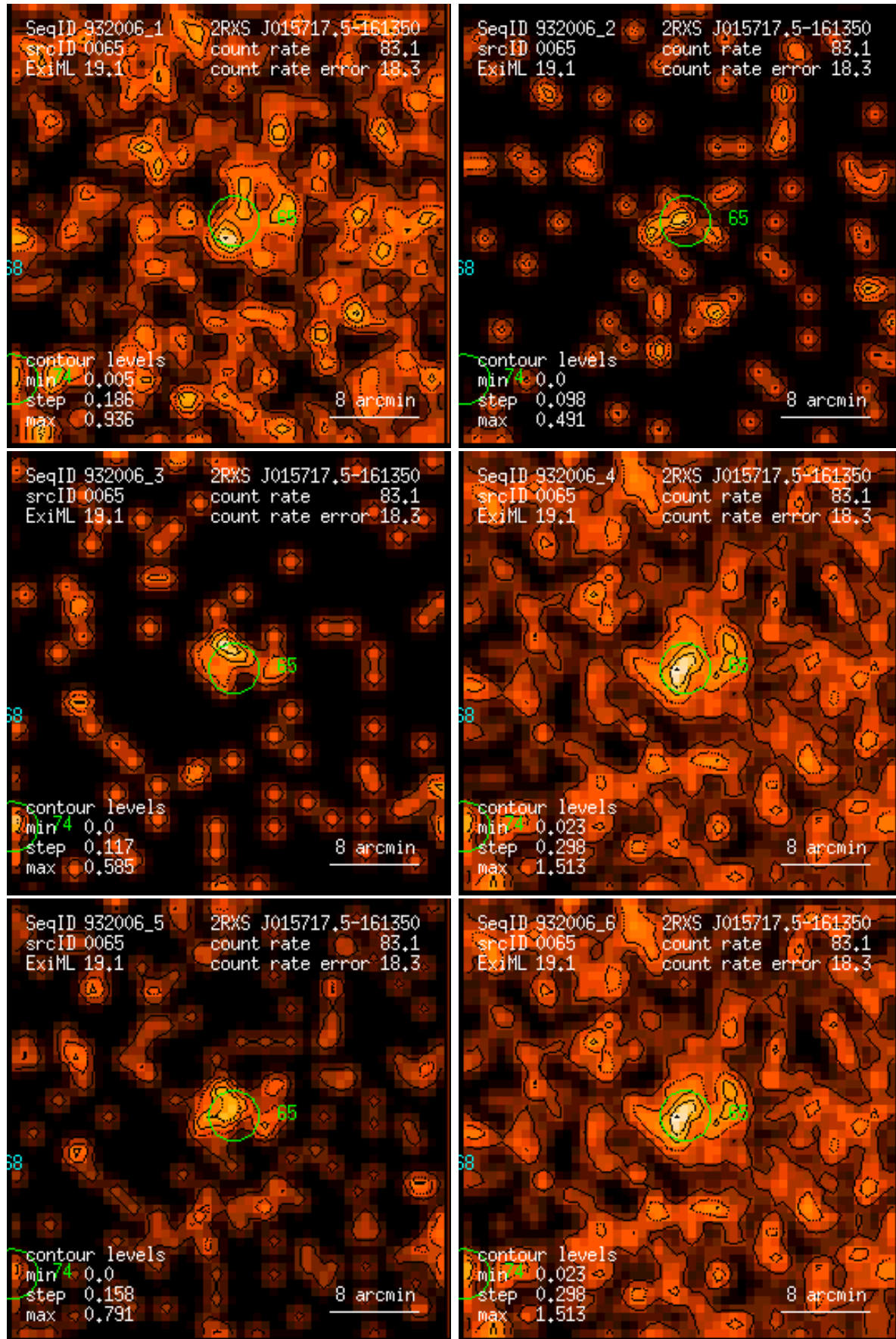
Figure 65: RASS 932006: detection 0065: band rate images, Gaussian filter: (1) PSPC channels 11 – 41, (2) 52 – 90, (3) 91 – 201, (4) 11 – 235, (5) 52 – 201, (6) 11 – 201. Broad band rates in counts/ks. Band rate contour levels in counts/ks/arcmin 2 .
