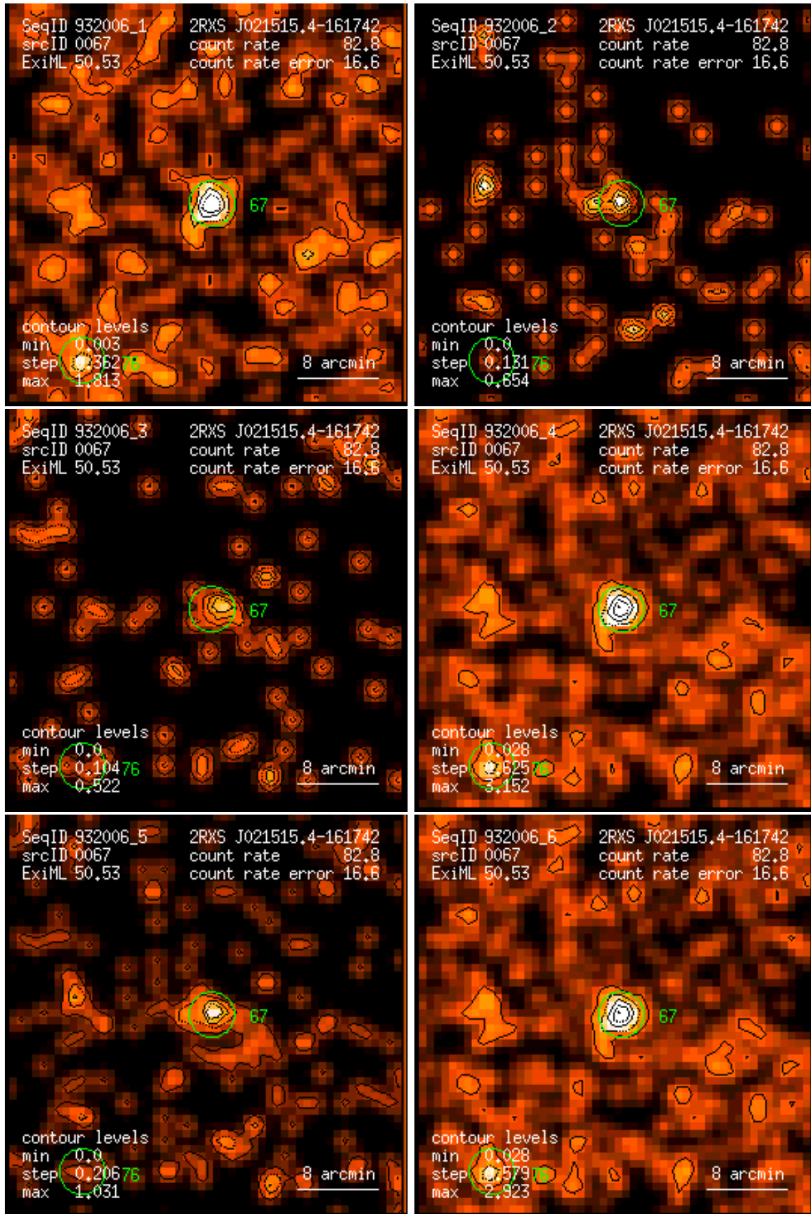
Figure 67: RASS 932006: detection 0067: band rate images, Gaussian filter: (1) PSPC channels 11 – 41, (2) 52 – 90, (3) 91 – 201, (4) 11 – 235, (5) 52 – 201, (6) 11 – 201. Broad band rates in counts/ks. Band rate contour levels in counts/ks/arcmin 2 .
