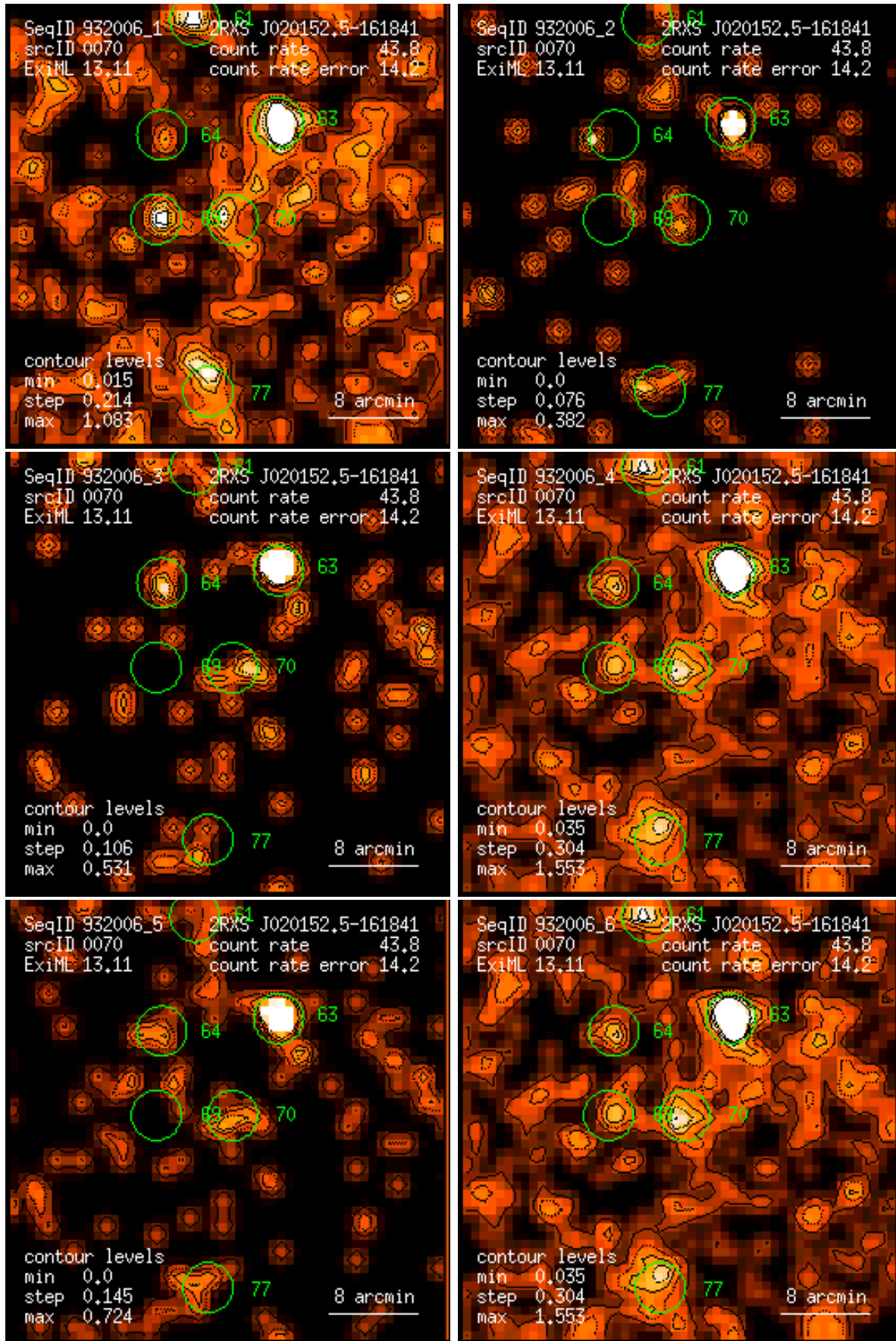
Figure 70: RASS 932006: detection 0070: band rate images, Gaussian filter: (1) PSPC channels 11 – 41, (2) 52 – 90, (3) 91 – 201, (4) 11 – 235, (5) 52 – 201, (6) 11 – 201. Broad band rates in counts/ks. Band rate contour levels in counts/ks/arcmin 2 .
