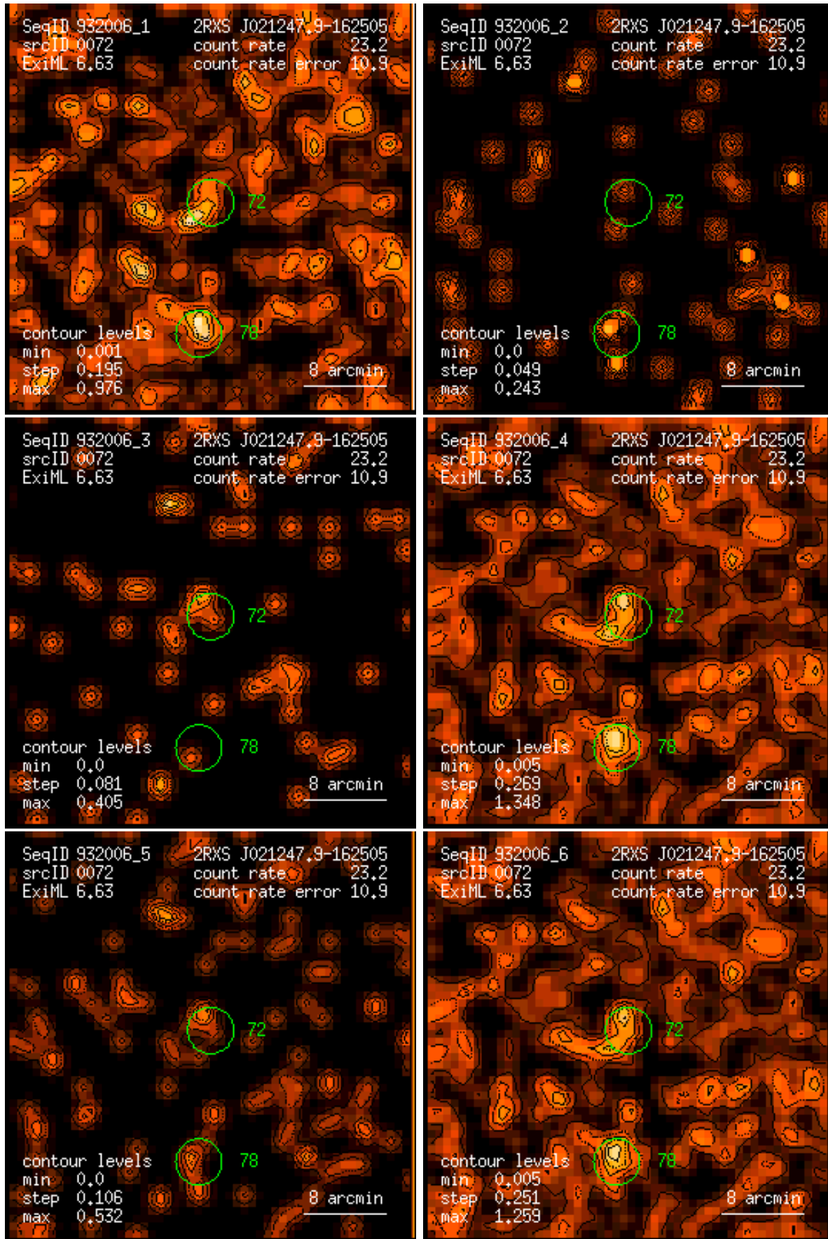
Figure 72: RASS 932006: detection 0072: band rate images, Gaussian filter: (1) PSPC channels 11 – 41, (2) 52 – 90, (3) 91 – 201, (4) 11 – 235, (5) 52 – 201, (6) 11 – 201. Broad band rates in counts/ks. Band rate contour levels in counts/ks/arcmin 2 .
