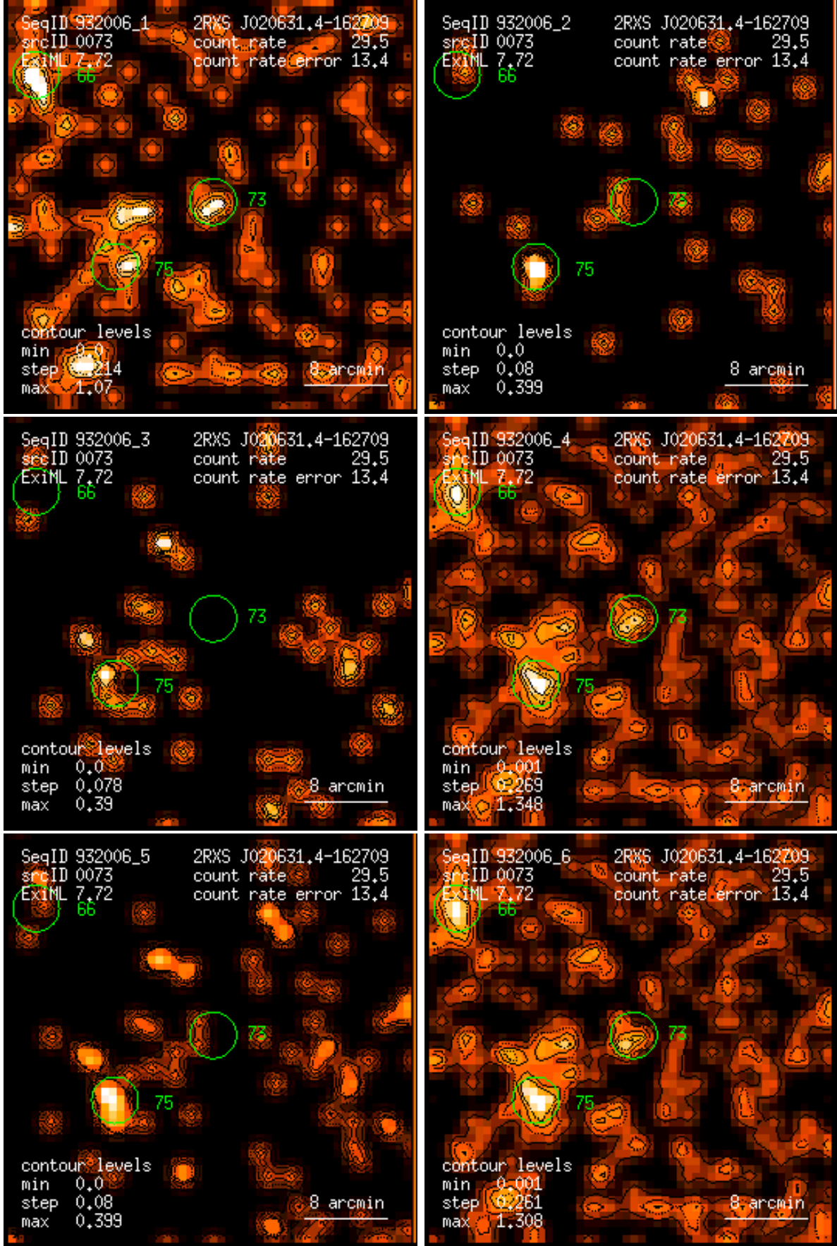
Figure 73: RASS 932006: detection 0073: band rate images, Gaussian filter: (1) PSPC channels 11 – 41, (2) 52 – 90, (3) 91 – 201, (4) 11 – 235, (5) 52 – 201, (6) 11 – 201. Broad band rates in counts/ks. Band rate contour levels in counts/ks/arcmin 2 .
