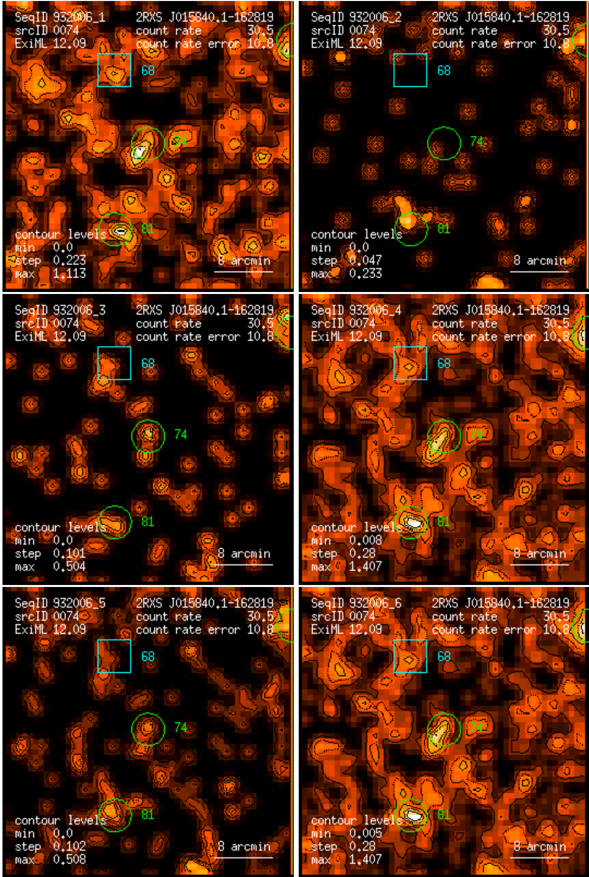
Figure 74: RASS 932006: detection 0074: band rate images, Gaussian filter: (1) PSPC channels 11 – 41, (2) 52 – 90, (3) 91 – 201, (4) 11 – 235, (5) 52 – 201, (6) 11 – 201. Broad band rates in counts/ks. Band rate contour levels in counts/ks/arcmin 2 .
