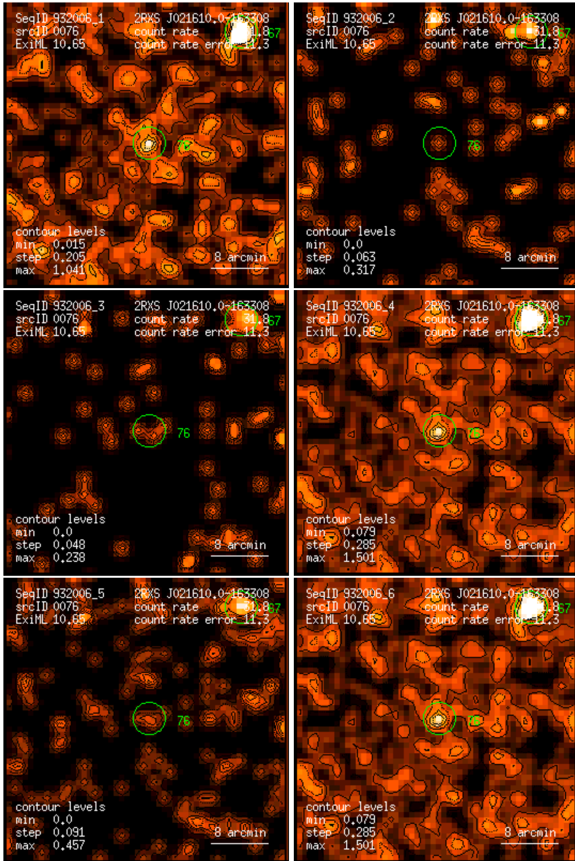
Figure 76: RASS 932006: detection 0076: band rate images, Gaussian filter: (1) PSPC channels 11 – 41, (2) 52 – 90, (3) 91 – 201, (4) 11 – 235, (5) 52 – 201, (6) 11 – 201. Broad band rates in counts/ks. Band rate contour levels in counts/ks/arcmin 2 .
