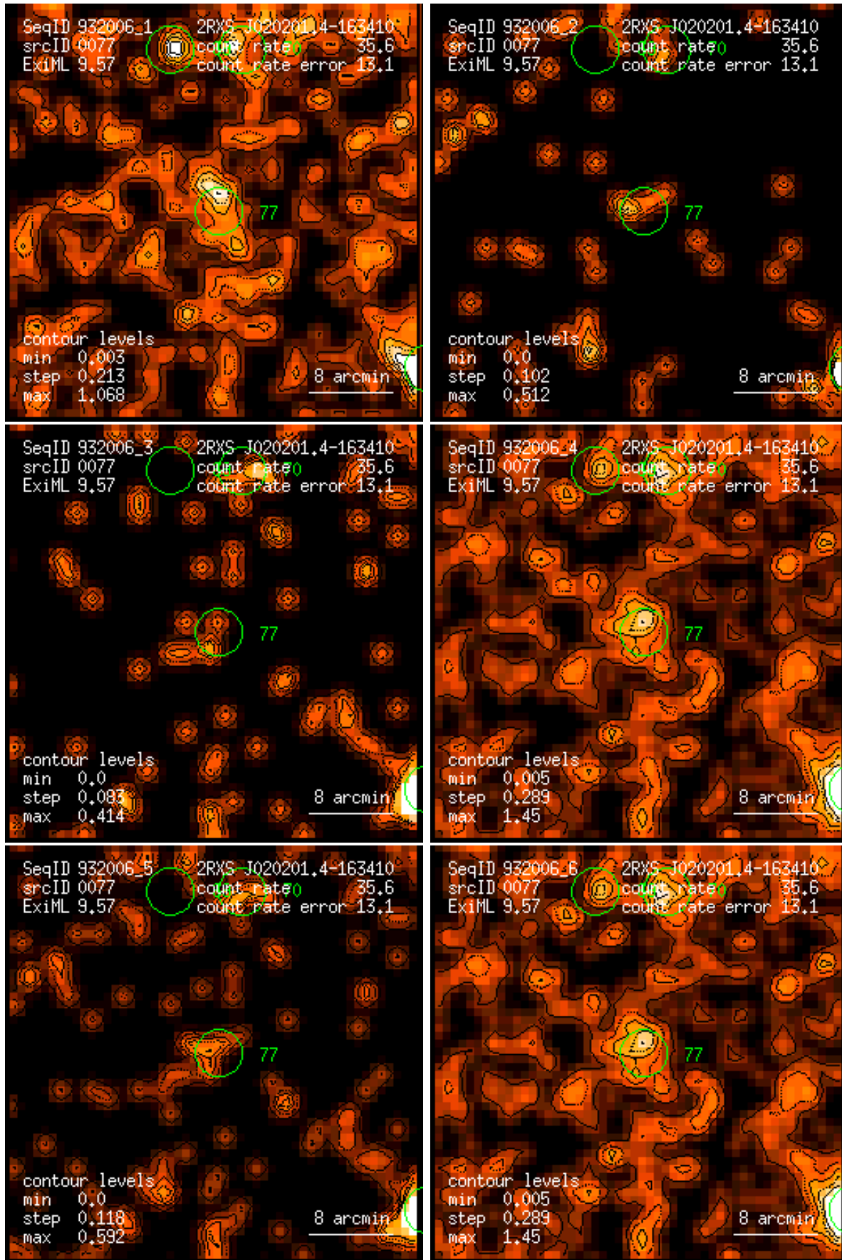
Figure 77: RASS 932006: detection 0077: band rate images, Gaussian filter: (1) PSPC channels 11 – 41, (2) 52 – 90, (3) 91 – 201, (4) 11 – 235, (5) 52 – 201, (6) 11 – 201. Broad band rates in counts/ks. Band rate contour levels in counts/ks/arcmin 2 .
