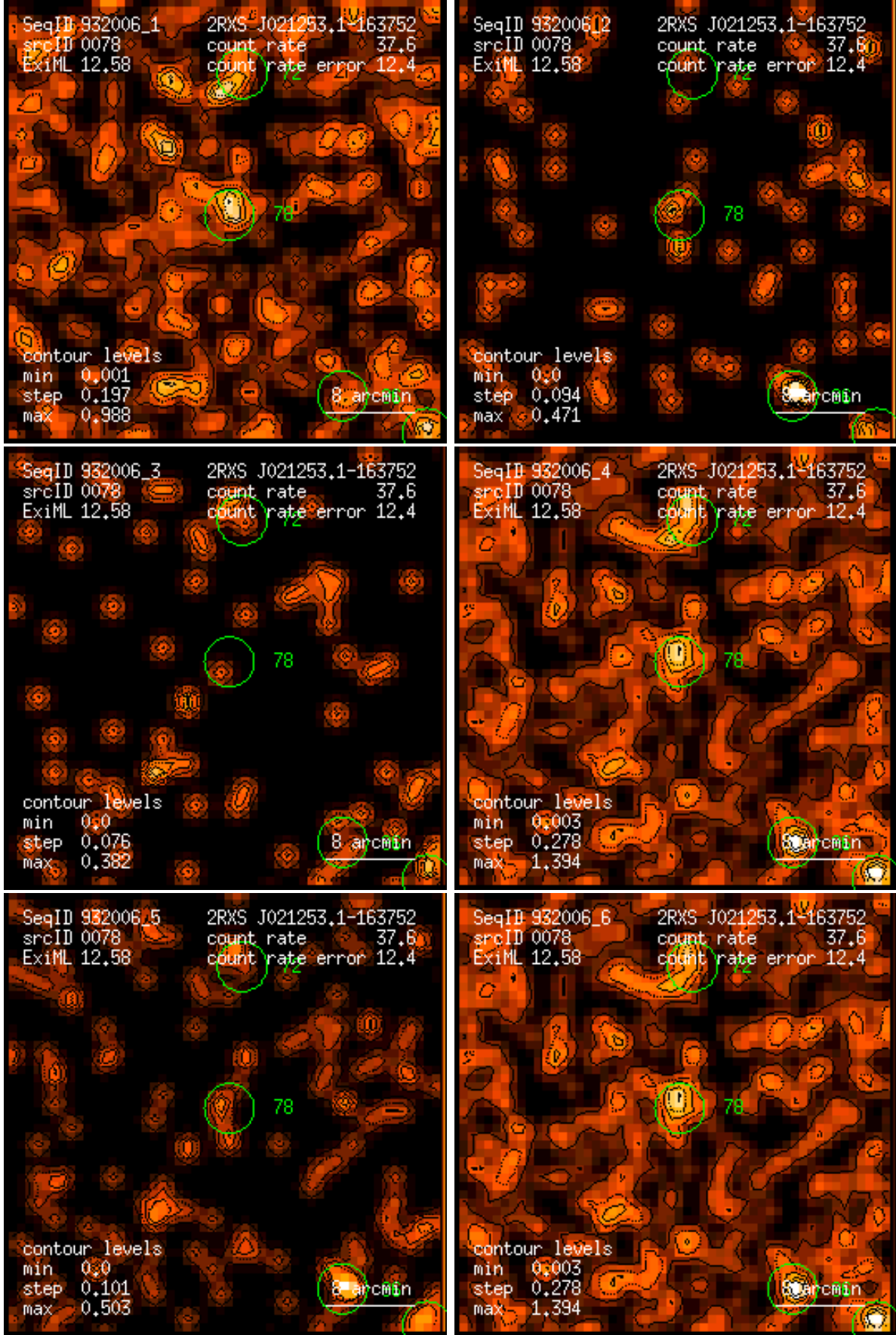
Figure 78: RASS 932006: detection 0078: band rate images, Gaussian filter: (1) PSPC channels 11 – 41, (2) 52 – 90, (3) 91 – 201, (4) 11 – 235, (5) 52 – 201, (6) 11 – 201. Broad band rates in counts/ks. Band rate contour levels in counts/ks/arcmin 2 .
