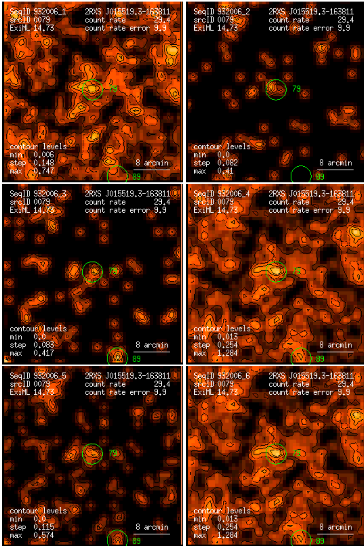
Figure 79: RASS 932006: detection 0079: band rate images, Gaussian filter: (1) PSPC channels 11 – 41, (2) 52 – 90, (3) 91 – 201, (4) 11 – 235, (5) 52 – 201, (6) 11 – 201. Broad band rates in counts/ks. Band rate contour levels in counts/ks/arcmin 2 .
