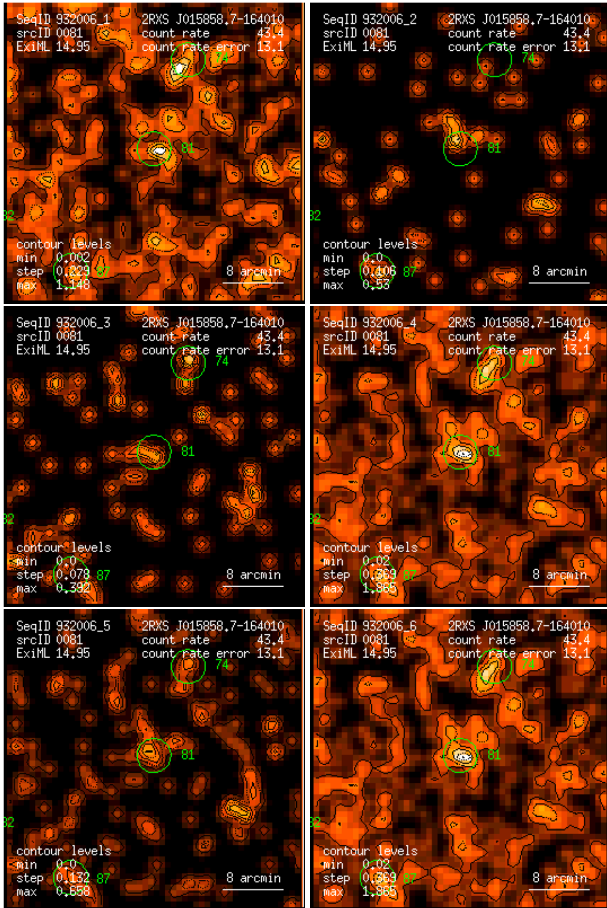
Figure 81: RASS 932006: detection 0081: band rate images, Gaussian filter: (1) PSPC channels 11 – 41, (2) 52 – 90, (3) 91 – 201, (4) 11 – 235, (5) 52 – 201, (6) 11 – 201. Broad band rates in counts/ks. Band rate contour levels in counts/ks/arcmin 2 .
