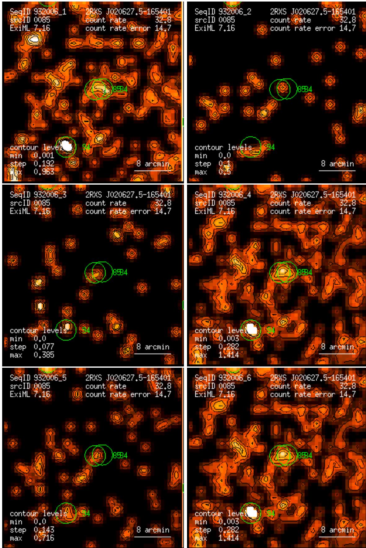
Figure 85: RASS 932006: detection 0085: band rate images, Gaussian filter: (1) PSPC channels 11 – 41, (2) 52 – 90, (3) 91 – 201, (4) 11 – 235, (5) 52 – 201, (6) 11 – 201. Broad band rates in counts/ks. Band rate contour levels in counts/ks/arcmin 2 .
